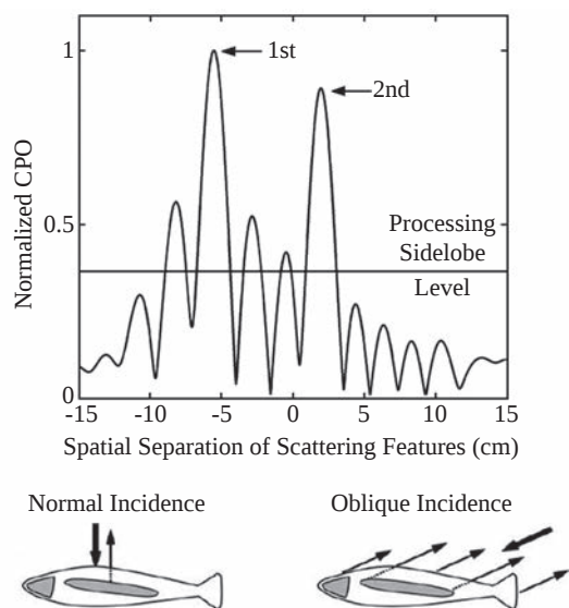
Fig. 3. Envelope of normalized compressed pulse output (CPO) for a fish at approximately 30° from tail-on orientation in the lateral plane (single-ping realization). The time delay on the horizontal axis has been converted to distance (cm) to represent the spatial separation between the scattering features of the fish, using the equation: \text{separation} = (\text{time delay}) * c / (2 \cos(\beta)) , where \beta is the angle of orientation relative to the transducer beam and c is the speed of sound. The processing sidelobe is an artifact of the pulse compression process; therefore, any peak significantly higher than the processing sidelobe level represents a physical arrival from the fish. From Reeder et al. [13].
