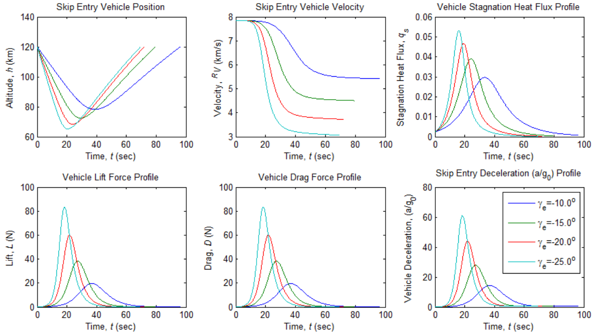
Figure 17. Variable Flight-Path Angle Simulation for Notional Satellite ( h = 120 km, L/D = 1.0 )
