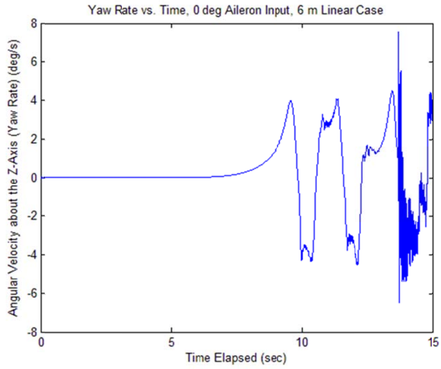
Figure 79. Case 1 Yaw Rate \omega_z versus Time
