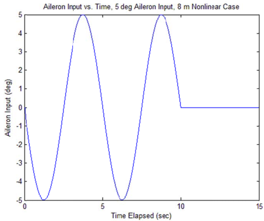
Figure 140. Case 11 Aileron Input versus Time
