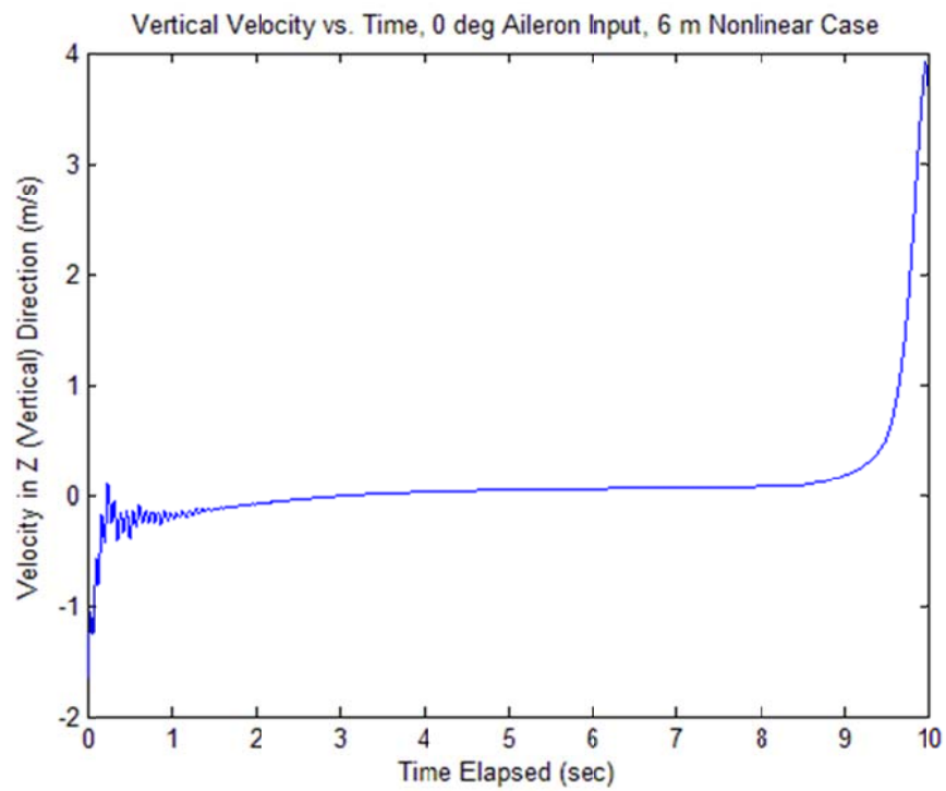
Figure 22. Case 3 Vertical Velocity v_z versus Time
