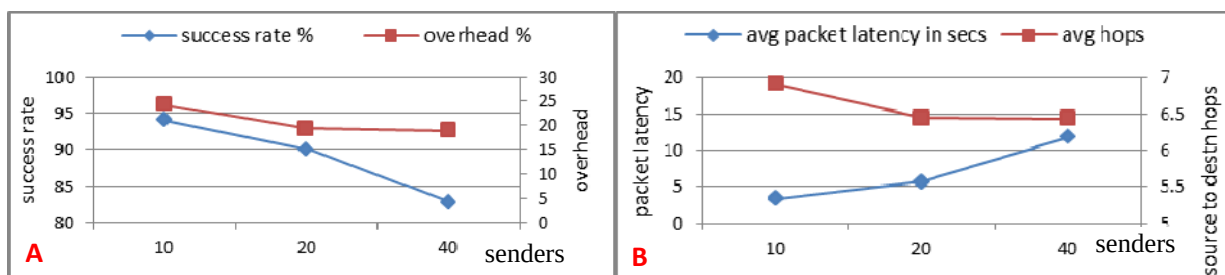
Figure 36 Performance Graphs – 50-Node Scenario (airborne backbone/directional)
