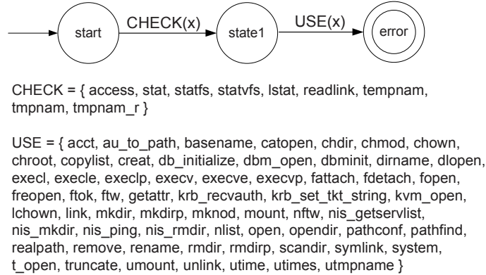
Figure 2: Race Condition Automaton (TOCTOU).
