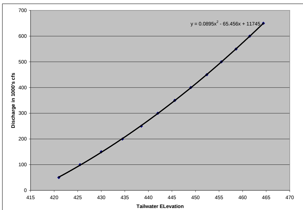
Figure 2.7. Markland Dam tailwater rating curve from model report.
