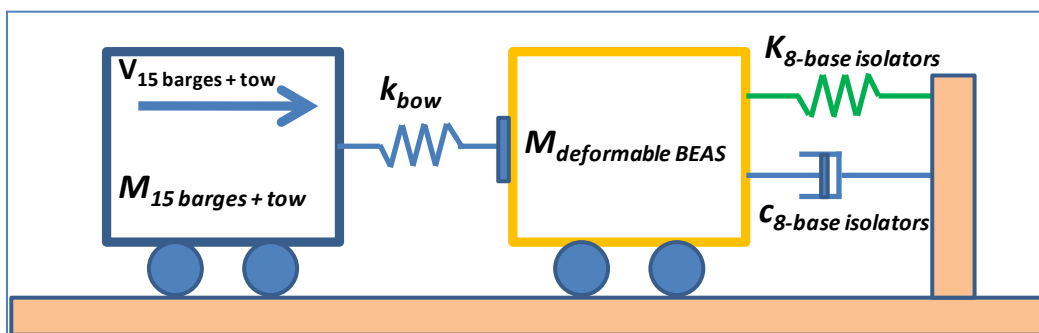
Figure 3.12 2-DOF system of the super-barge dBEAS model.
