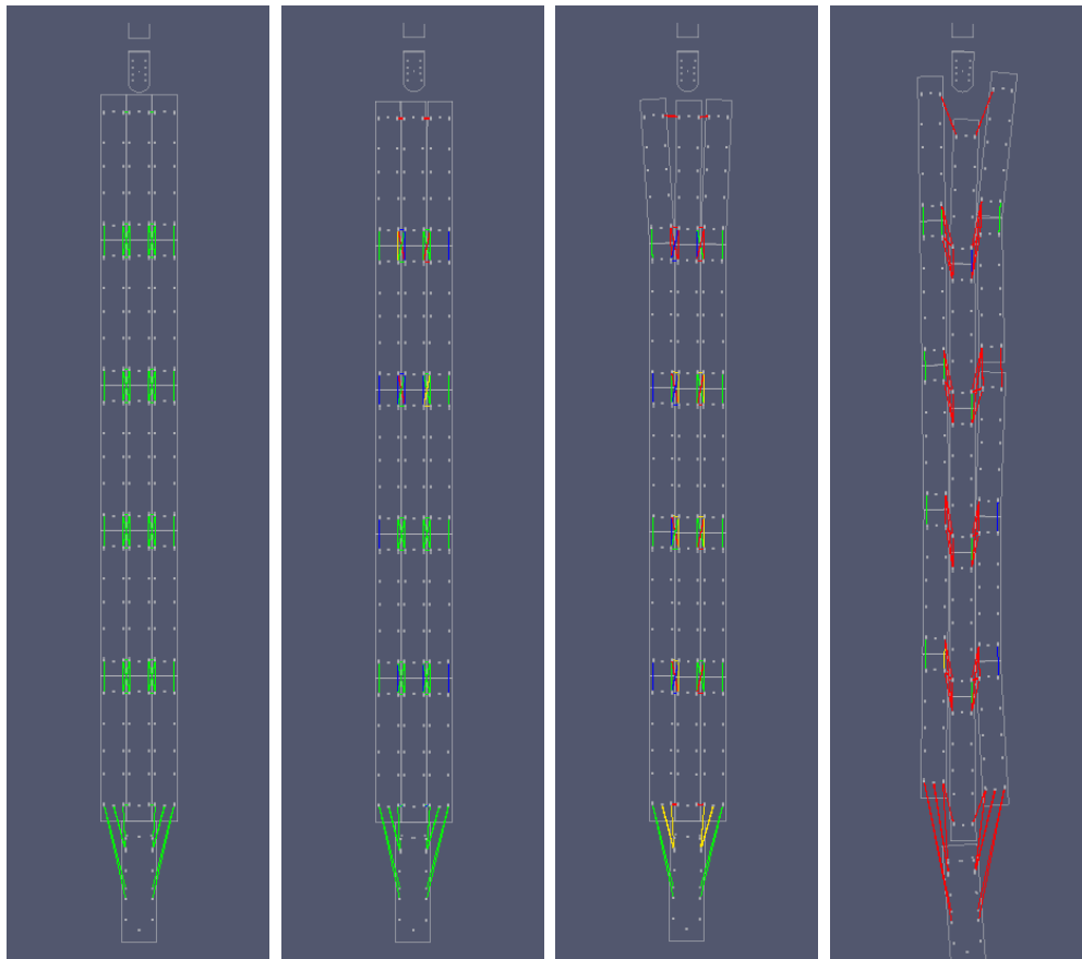
Figure 3.20 Barge train velocity tests at time=10 sec: (a) 2fps - no lashings broken, (b) 4fps - lashings broken (c) 4.5fps - strained but barge train integrity maintained, and (d) 6fps - barge train integrity lost.
