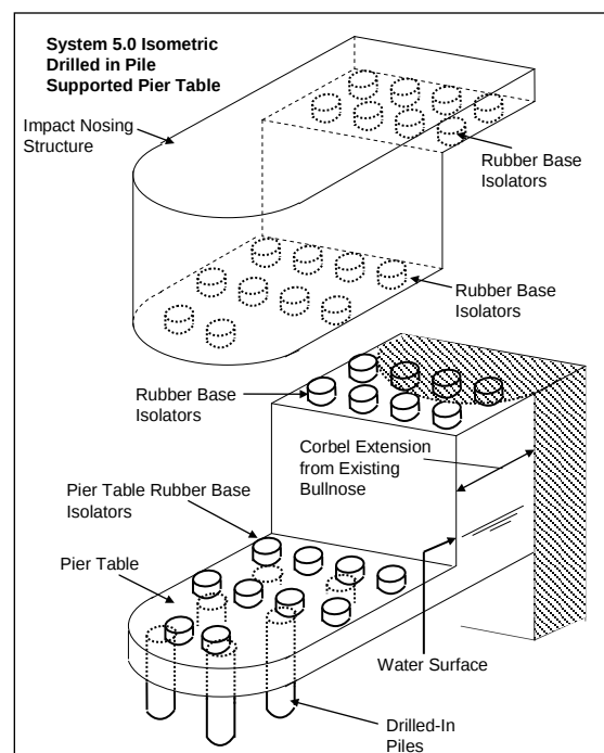
Figure 1.1 Fixed Corbel extension single impact nosing.
