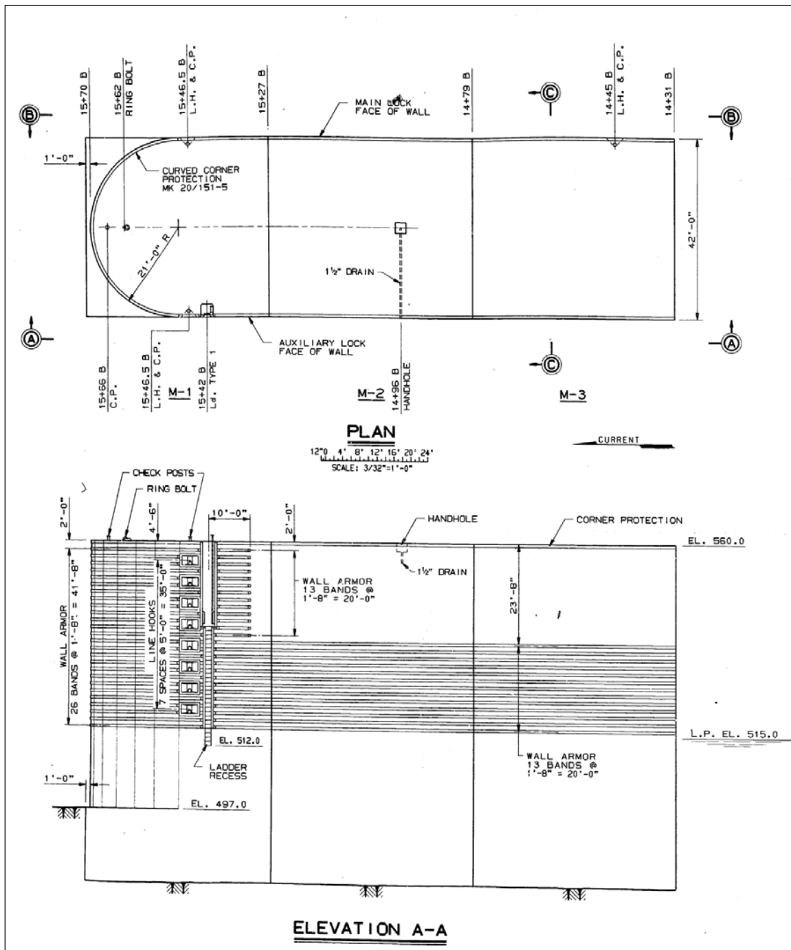
Figure 5.15 Downstream design for the R.C. Byrd center wall
