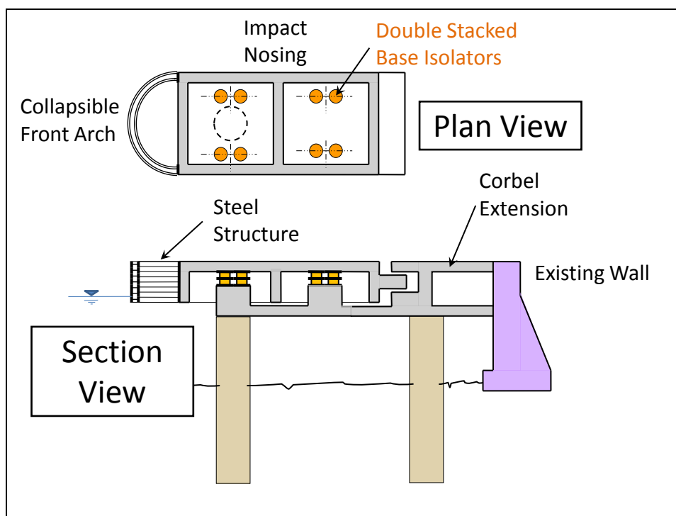
Figure 4.1 A single-part impact nosing with stacked base isolators and collapsible front arch.
