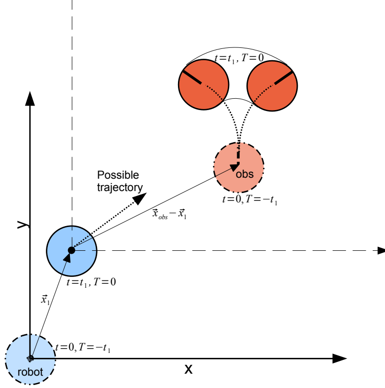
Figure 4-2: For a general coordinate \vec{x}_1 that is reached by the host robot at time t_1 , a time-shifted VOS can be computed for each obstacle that determines the safety of single-velocity trajectories originating from \vec{x}_1 for times t > t_1 . It is convenient to define a new time-frame T = t - t_1 such at T = 0 , that the host robot is at \vec{x}_1 and the reachable set of the obstacle has already grown out of its initial location by t_1 seconds. The time-shifted VOS is computed the same way as detailed in Chapter 3 using these reachable sets for all T > 0 .
