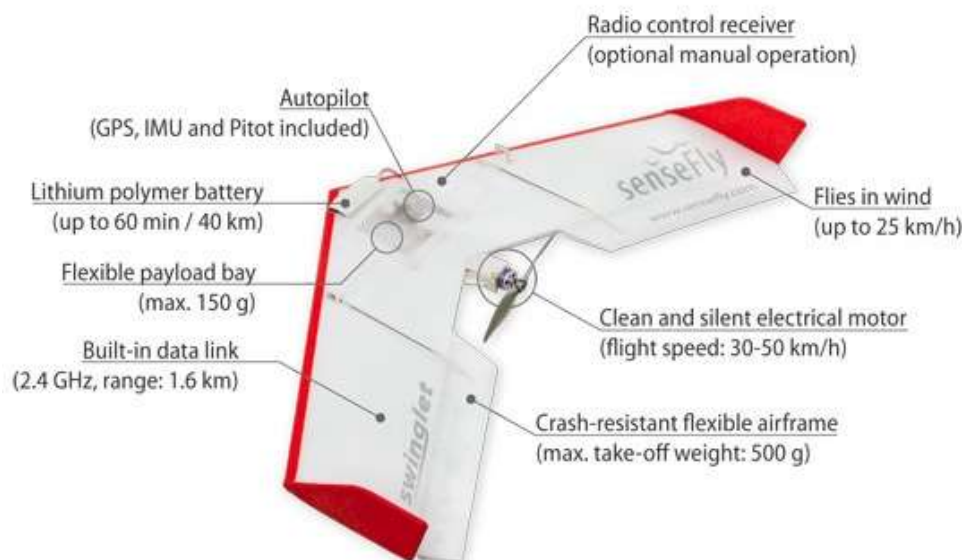
Figure 5 - senseFly's swinglet
