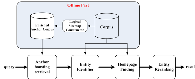
Figure 4: the Related Entity Finding System Architecture.
