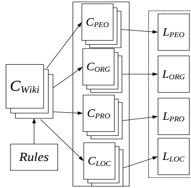
Figure 3. Build entity lists of four types.
