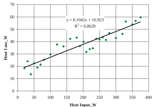
Figure 8: Heat loss to ambient
