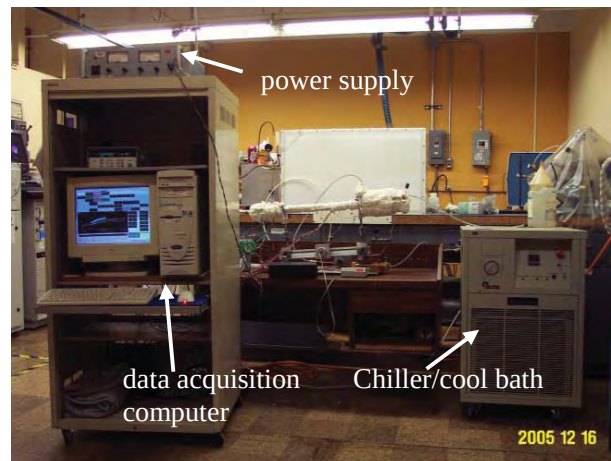
Figure 3: Test setup
