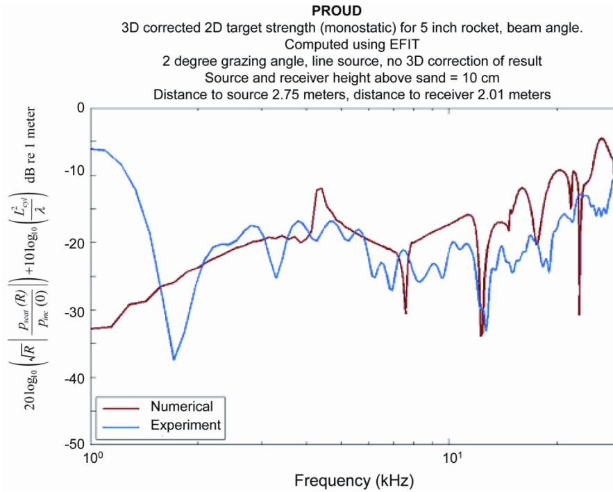
Figure 33b – Target Strength versus Frequency.
