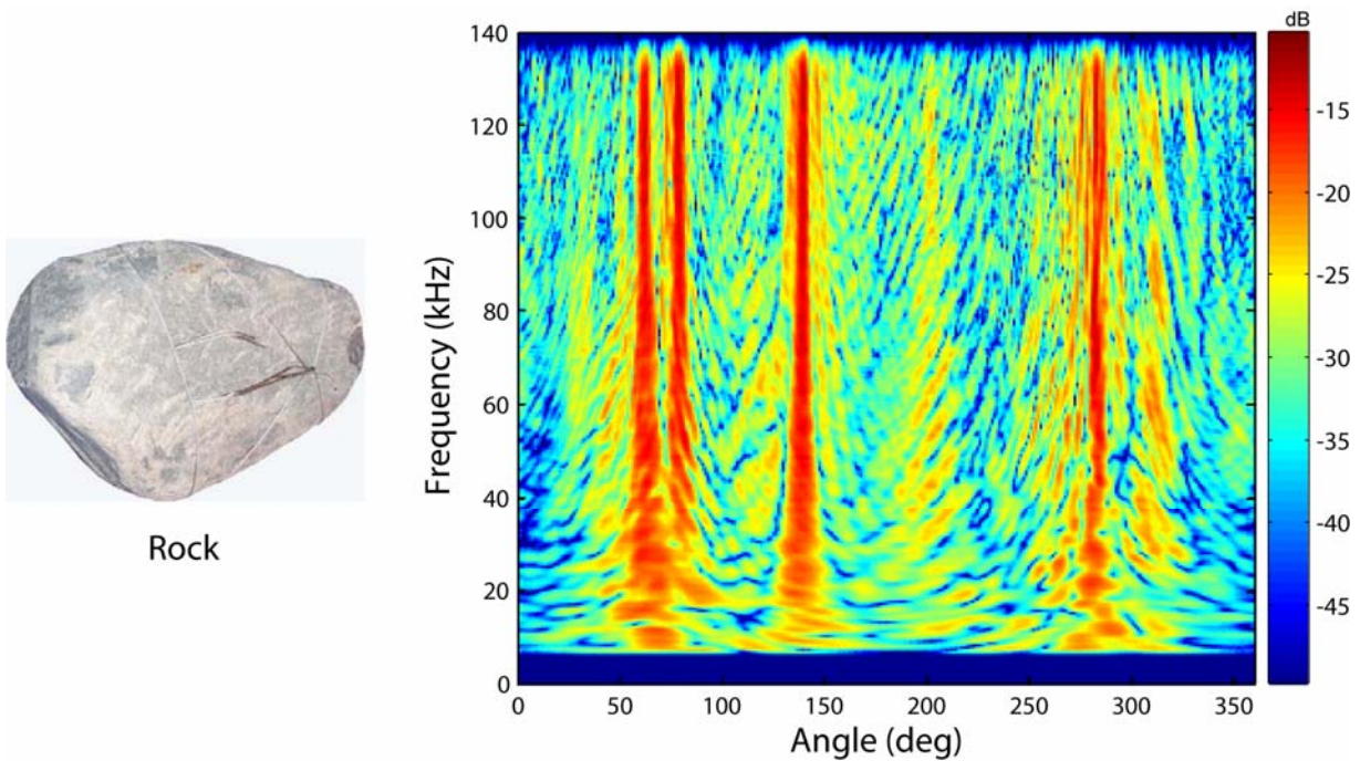
Figure 11 – Measured Target Strength & Target Photo.
