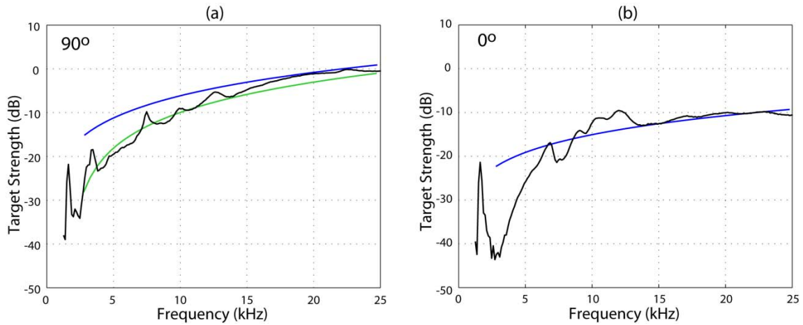
Figure 40 – Measured Forward Scattering TS Versus Analytic Model.
