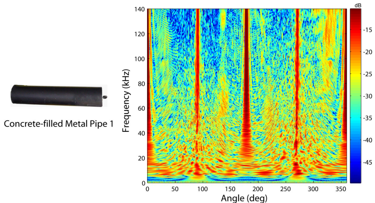
Figure 12 – Measured Target Strength & Target Photo.
