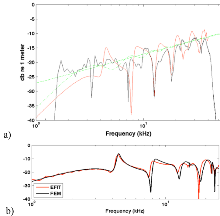
Figure 31 – Target Strength versus Frequency for Infinite Cylindrical Shell with Five Inch Rocket Parameters.
