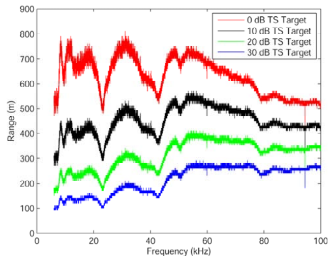
Figure 14 – Maximum Detection Range versus Frequency. Maximum distance that a target could be detected ( S/N = 1 ) for a medium without boundaries, noise spectral levels measured in the San Diego Harbor, and a source level of 170 dB re: \mu Pa.
