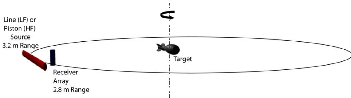
Figure 3 – Experimental Measurement Geometry
