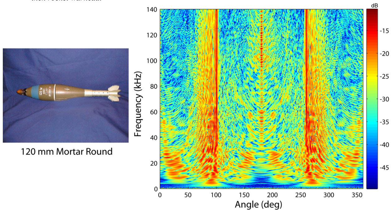
Figure 7 – Measured Target Strength & Target Photo.
