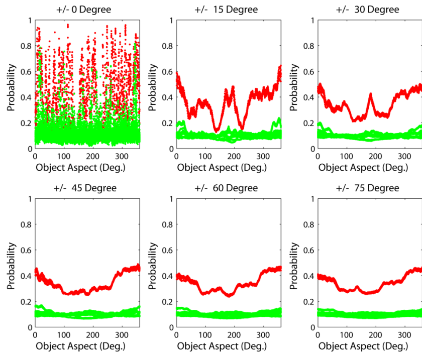
Figure 21 – Probability for Correct Target Identification.
