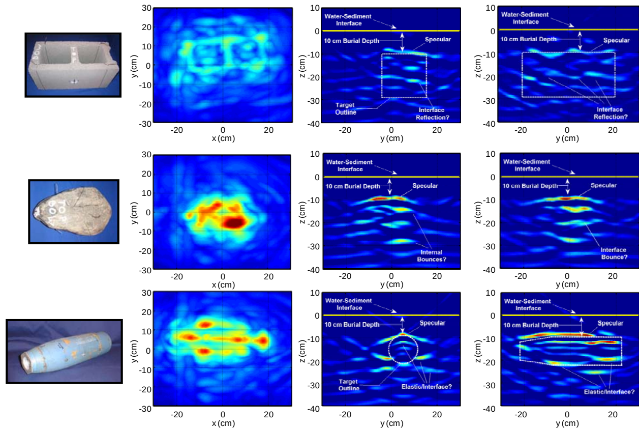
Figure 60 – Buried Target Images. Three different 2D planes: from left to right plan view, short side view, long side view.
