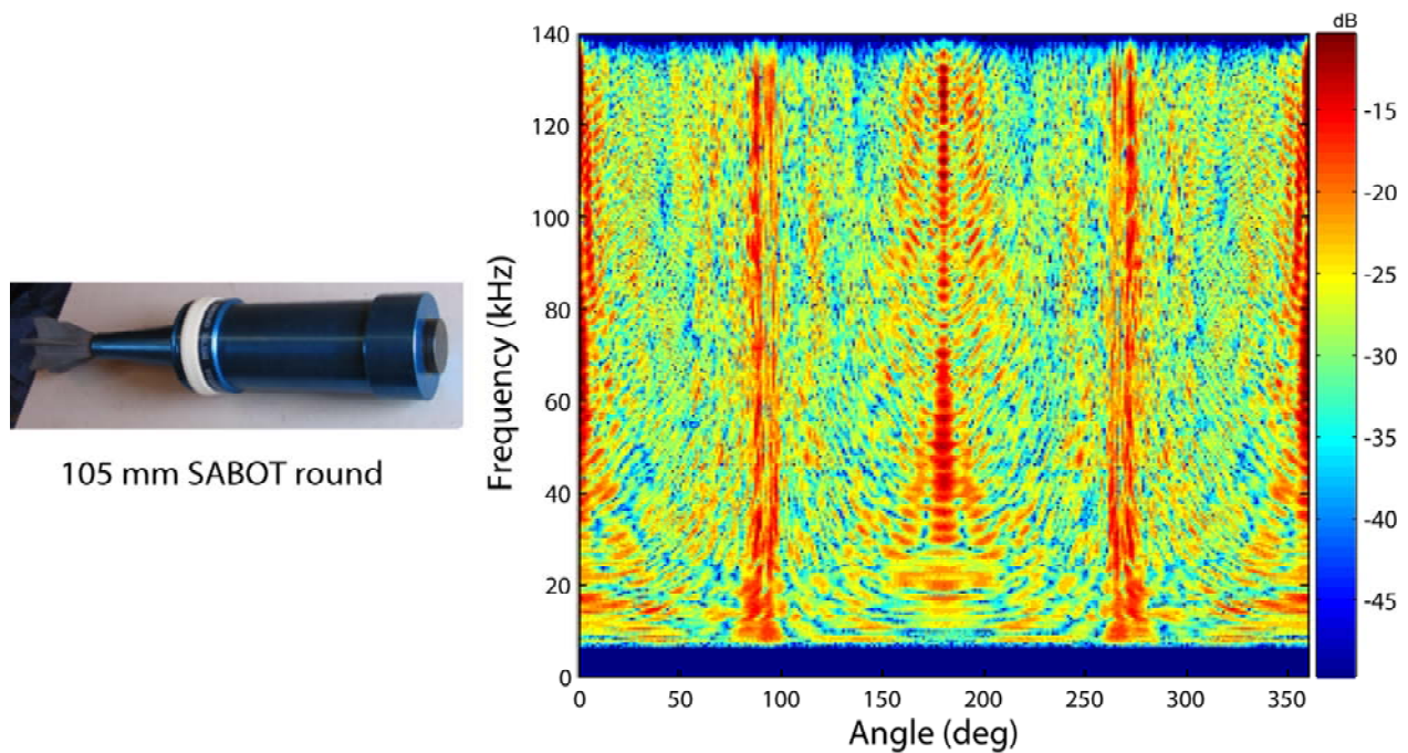
Figure 8 – Measured Target Strength & Target Photo.
