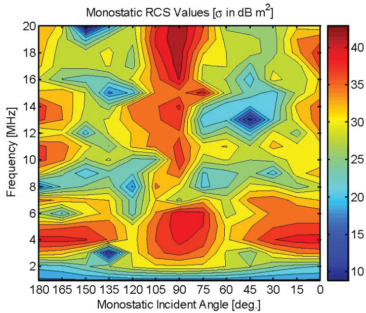
Figure 19: RCS values with a 5 deg rotational lift.
