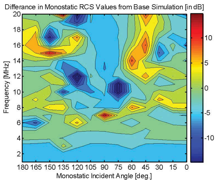
Figure 27: Difference from base simulation I ( \sigma_{4\text{ below}}/\sigma_{\text{base}} in dB).
