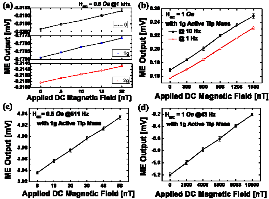
Figure. VIII.4. ME output voltage corresponding to an applied small DC magnetic field: (a) 5 nT under the constant condition of H_{ac}=0.5 \text{ Oe} at f=1 \text{ kHz} with/without active tip mass, (b) 300 nT under H_{ac}=1 \text{ Oe} at f=10 and 1 \text{ Hz} with 1g active tip mass, (c) and (d) ME response with a 1g active tip mass operating in the 2 nd and 1 st modes, (c) 10 nT under H_{ac}=0.5 \text{ Oe} at f=511 \text{ Hz} , (d) 2 \mu\text{T} under H_{ac}=0.5 \text{ Oe} at f=43 \text{ Hz} .
