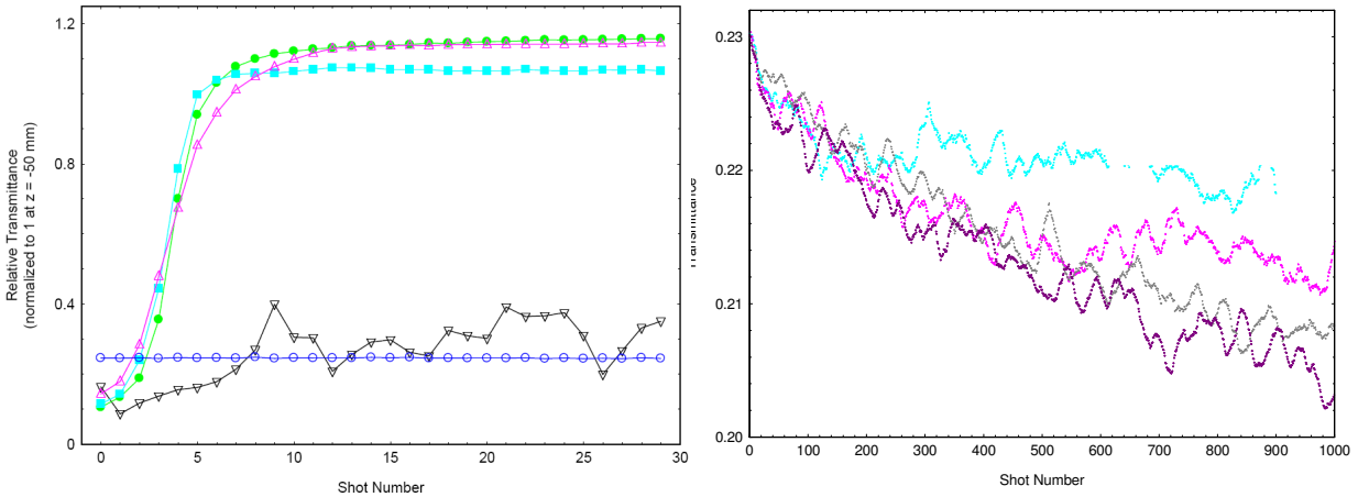
Figure 4. Transmission behavior of graphene based suspensions with successive laser shots. Blue circles in left plot represent the control sample.
