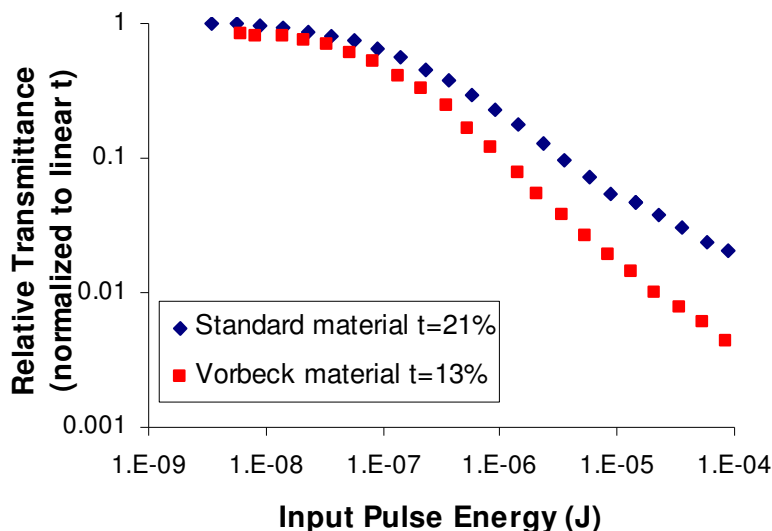
Figure 2. Non-linear optical limiting of Vorbeck solution versus state-of-the-art.
