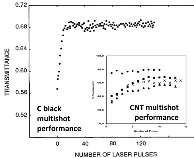
Figure 5. Example for literature of increase in transmission behavior of carbon black and carbon nanotubes (CNT) suspensions with successive laser shots. 23, 24
