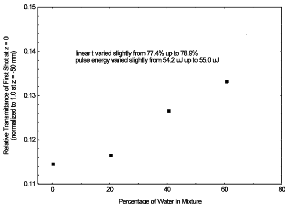
Figure 3. Effect of varying the ratio of water to isopropyl alcohol in graphene based suspensions. The linear transmittance was 78%.
