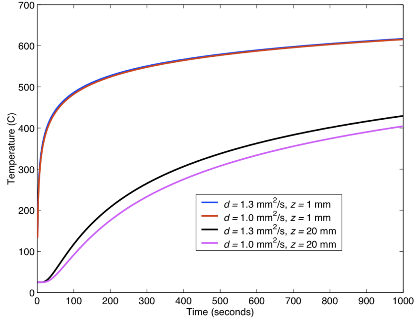
Figure 2.3: Transient Temperature Values at z = 1 mm and z = 20 mm at Different Times Due to Fast Transient Thermal Loadings
