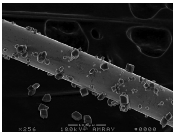
Figure 2 SEM image of AlH 3 on platinum filament.
