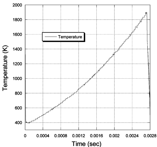
Figure 5 Typical temperature-time history for a heating rate of \sim 5 \times 10^5 \text{ K/s} .
