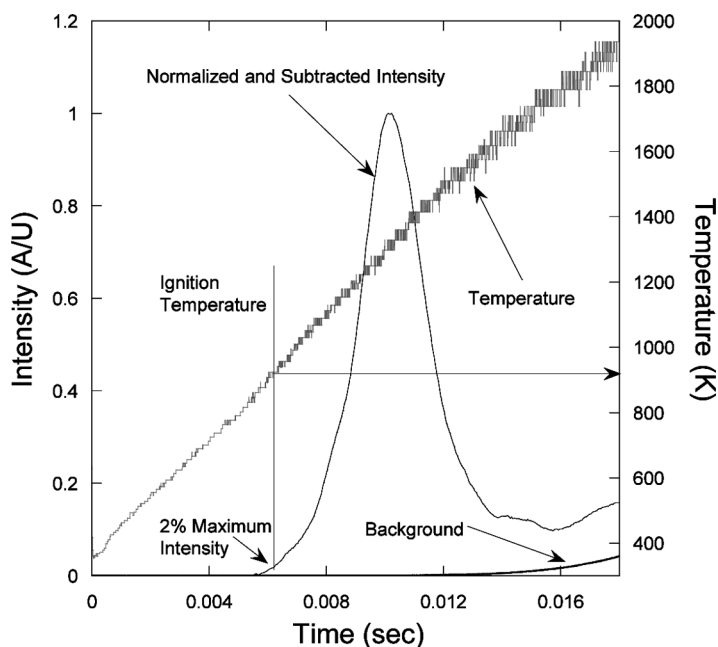
Figure 10 Example of the temporal temperature and optical emission for an \text{AlH}_3 ignition event.
