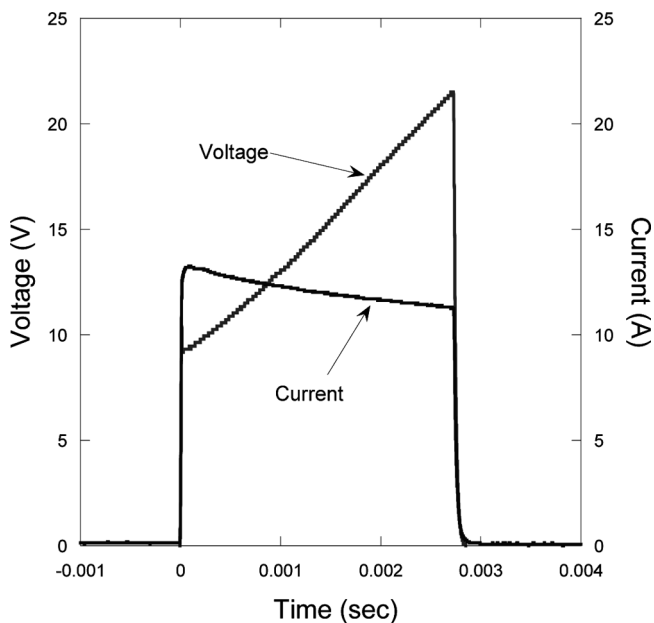
Figure 4 Typical voltage and current trace from 76 \mu\text{m} pt wire for heating rate of \sim 5 \times 10^5 \text{ K/s} .
