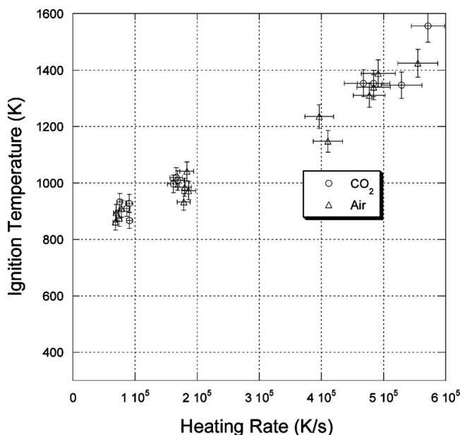
Figure 11 Ignition temperature of AlH 3 in air and CO 2 as a function of heating rate.
