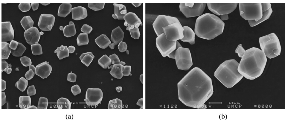
Figure 1 SEM images of AlH 3 .
