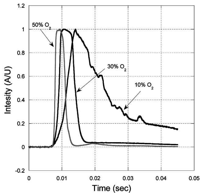
Figure 14 Temporal optical emission of combustion for various O 2 concentrations for a heating rate of \sim 7 \times 10^4 K/s.
