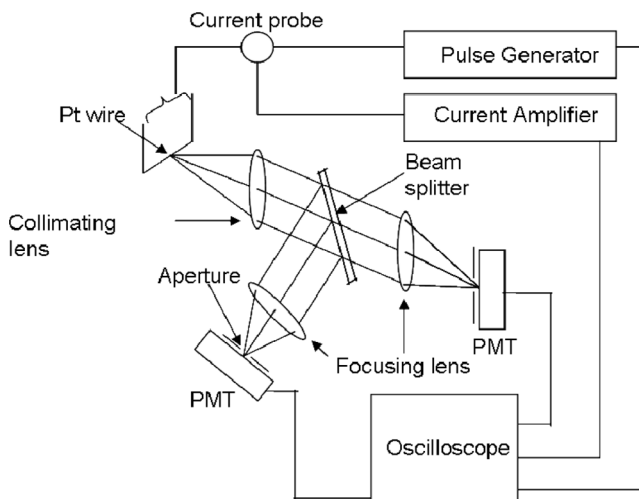
Figure 3 Schematic diagram of T-Jump optical emission system.
