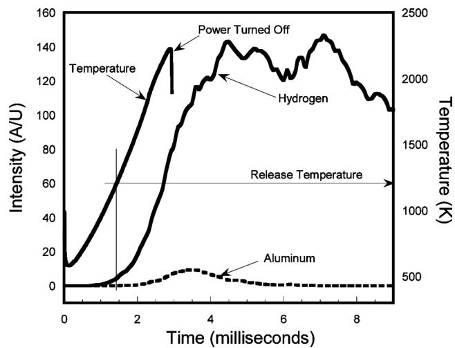
Figure 7 Hydrogen release for heating rate of \sim 6 \times 10^5 K/s.
