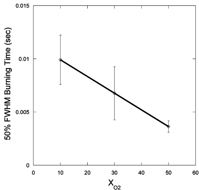
Figure 15 Burning time of AlH 3 as a function of O 2 concentration for a heating rate of \sim 6 \times 10^4 K/s.
