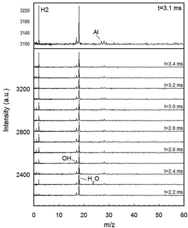
Figure 6 Temporally resolved T-Jump TOF mass spectra for a heating rate of \sim 6 \times 10^5 K/s.
