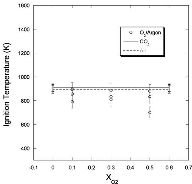
Figure 13 Ignition temperature of AlH 3 in Ar/O 2 Mixtures for a heating rate of \sim 7 \times 10^4 K/s.
