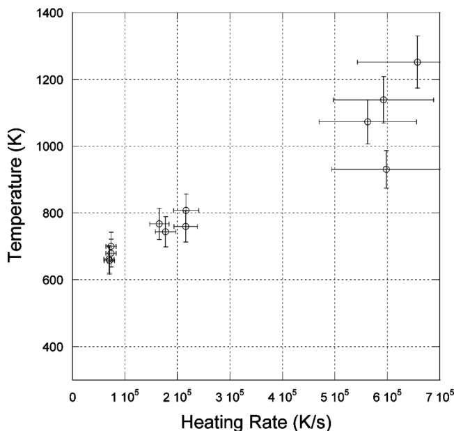
Figure 8 Hydrogen release temperature from AlH 3 as a function of heating rate.
