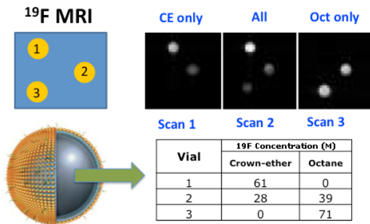
Figure 6. Selective MRI of ^{19}\text{F} nanoemulsions of perfluoro- 15-crown-ether and perfluoro-octane
