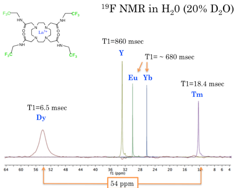
Figure 5. The effect on lanthanide selection on the Resonance Frequency of the \text{CF}_3 group
