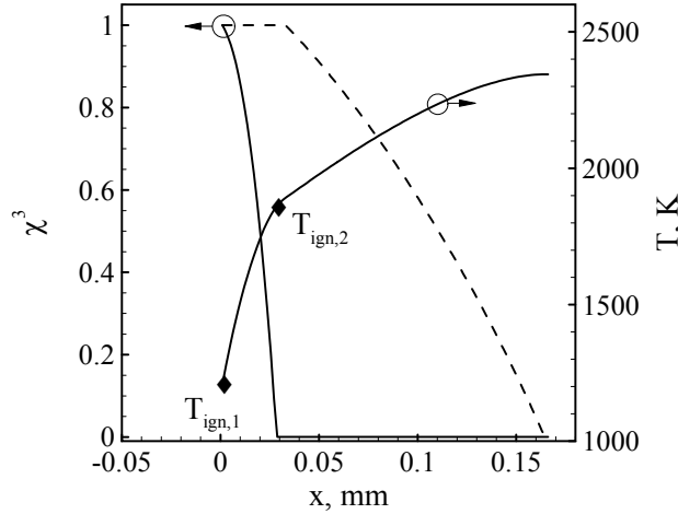
Figure 47: Temperature and particle mass consumption profiles of bimodal Al-Alane-ice mixtures at 7 MPa.
