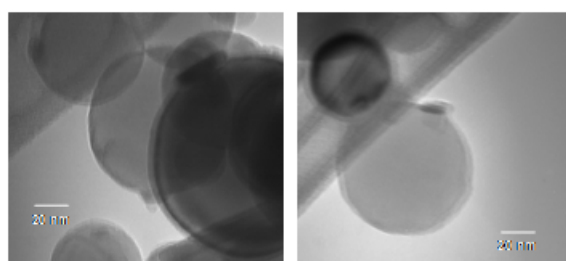
Figure 3: TEM photographs of 80-nm Al without (left) and with (right) additional passivation.
