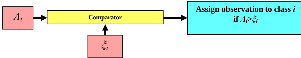
Figure 9. Bayesian Classifier
