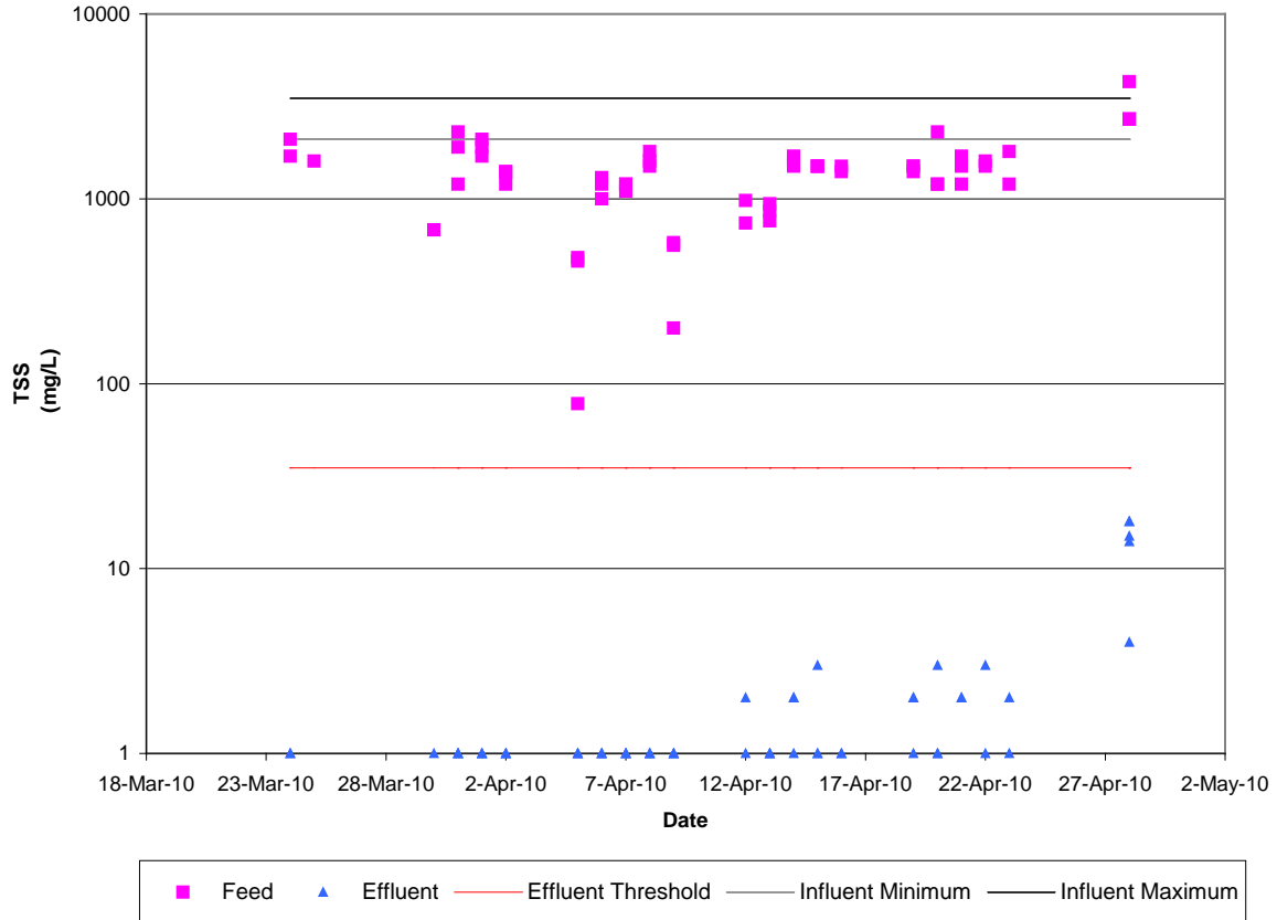
Figure 23. Graph of Analytical Results for TSS for Phase 2
