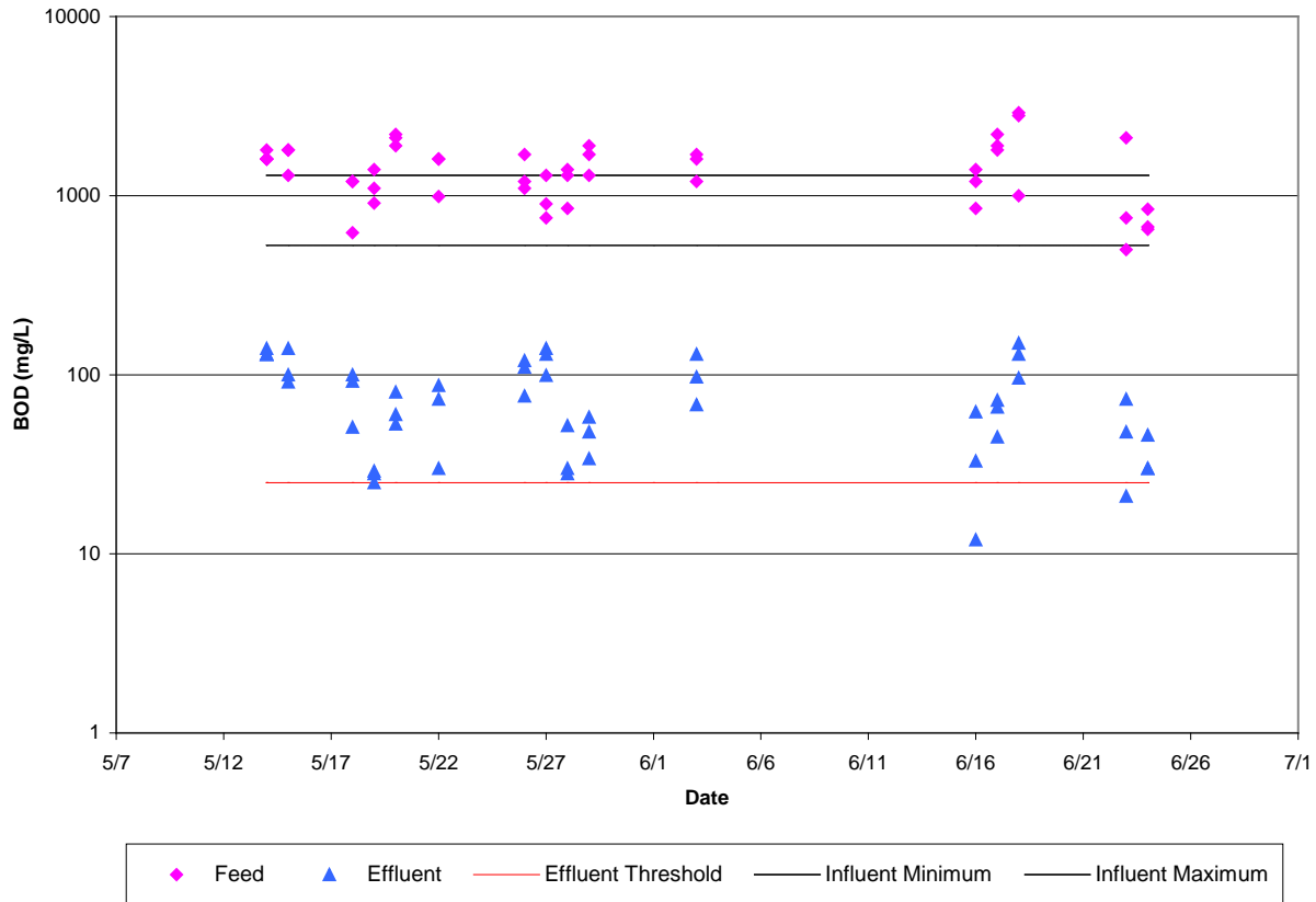
Figure 16. Graph of Analytical Results for BOD 5 for Phase 1
