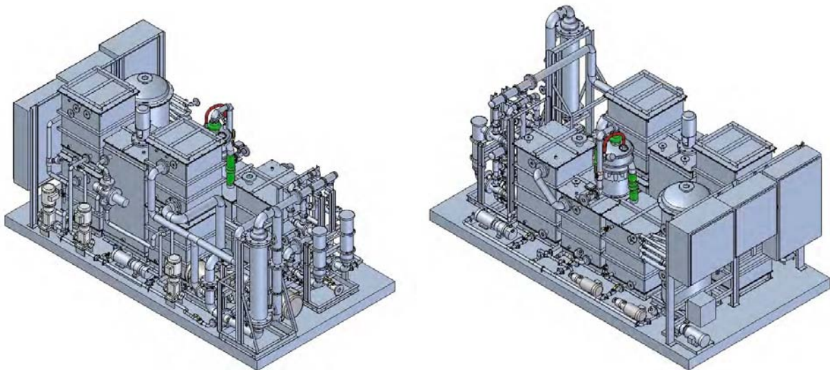
Figure 3. Navalis Orion™ Advanced Oxidation Wastewater Treatment System Right Front Isometric View and Left Rear Isometric View
