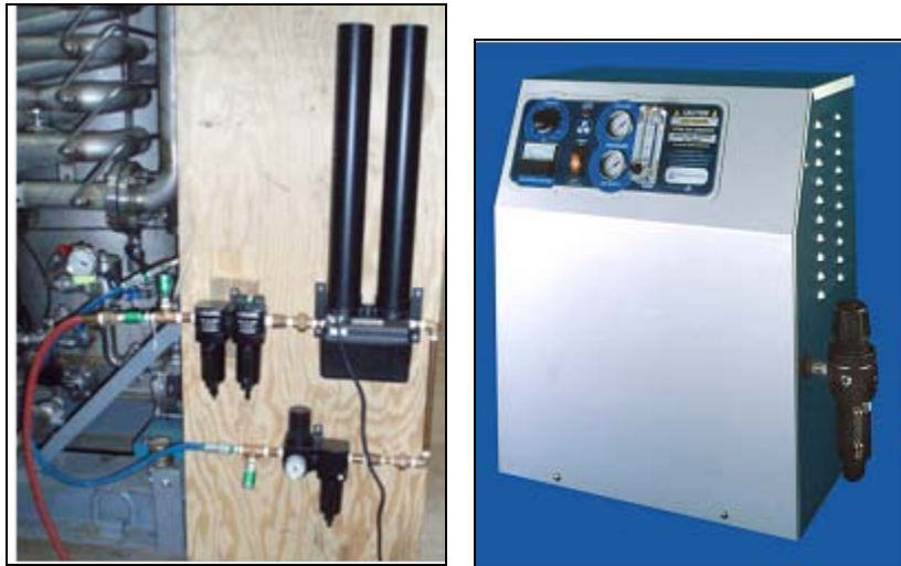
Figure 10. Photos of Twin Engineering Desiccant Air Dryer and Ozone Generator
