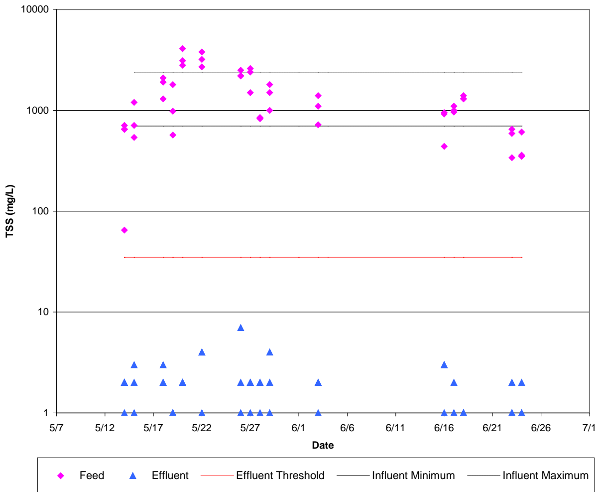
Figure 18. Graph of Analytical Results for TSS for Phase 1
