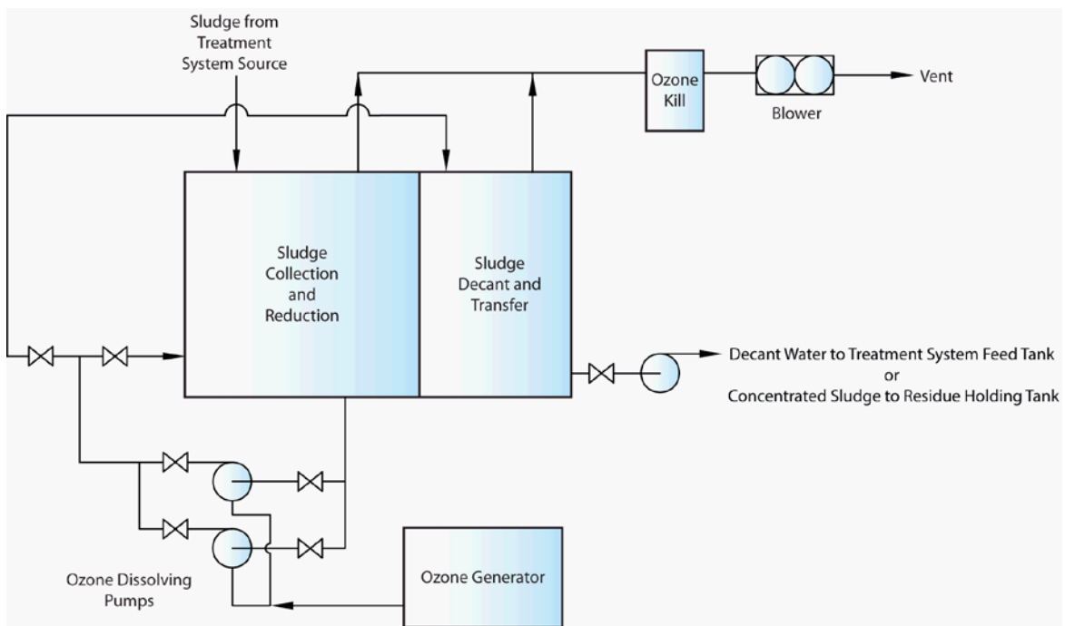
Figure 2. Sludge Reduction and Management System Process Flow Diagram
