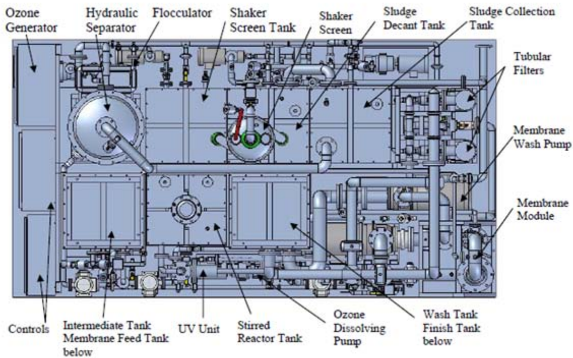
Figure 5. Aerial Isometric View of the Navalis Orion™ Advanced Oxidation Wastewater Treatment System
