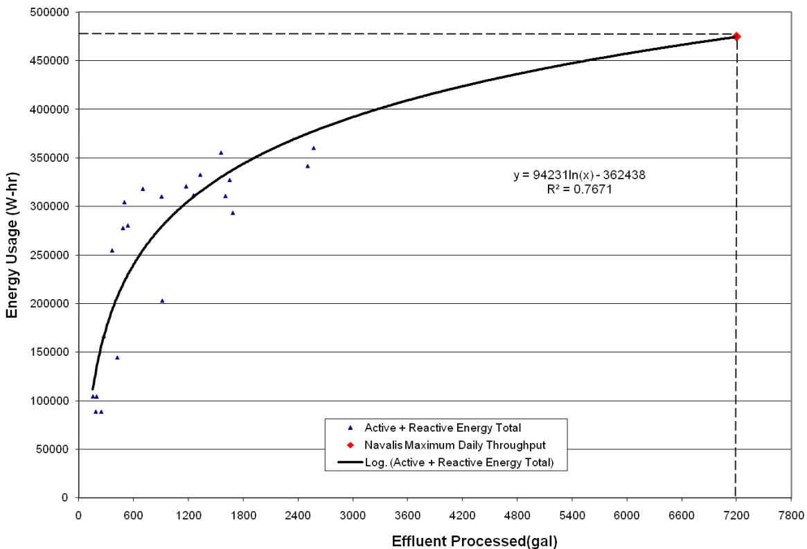
Figure 26. Graph of Energy Usage versus Effluent Processed
