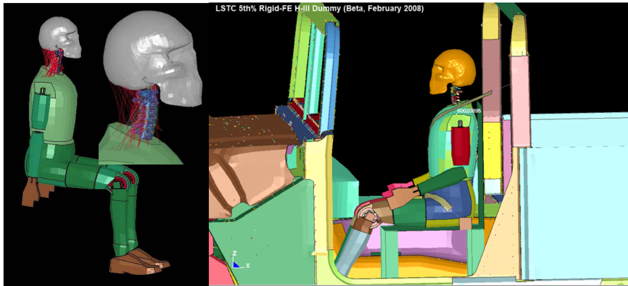
Figure 9. The High Fidelity Head Combined with the Hybrid III FEM and Included in the HMMWV Model
