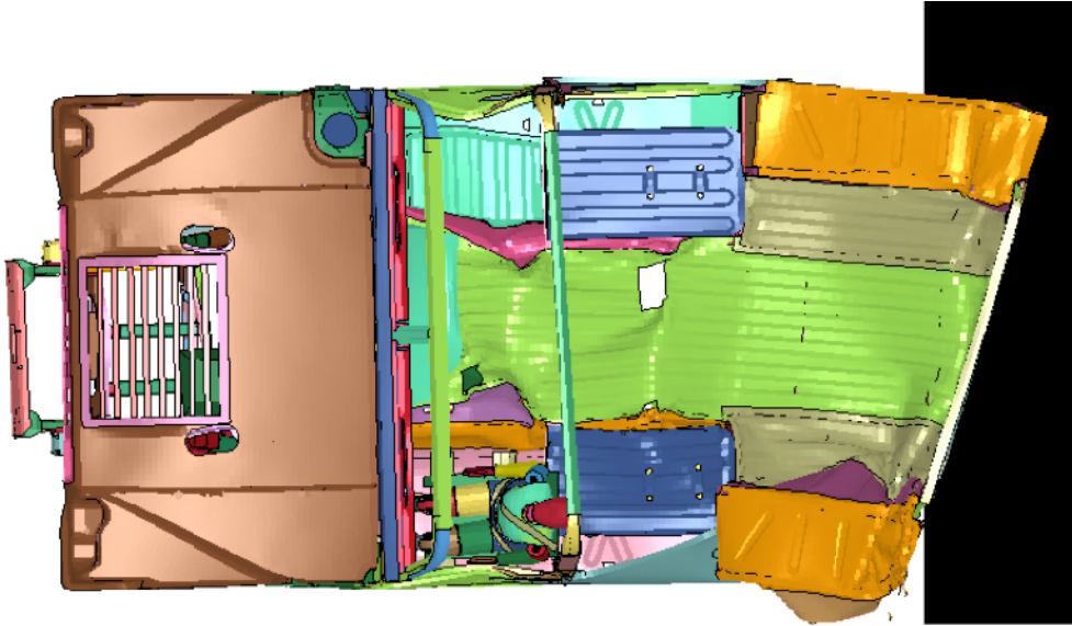
Figure 30. Top view of an angled rear impact of a HMMWV with a rigid wall
