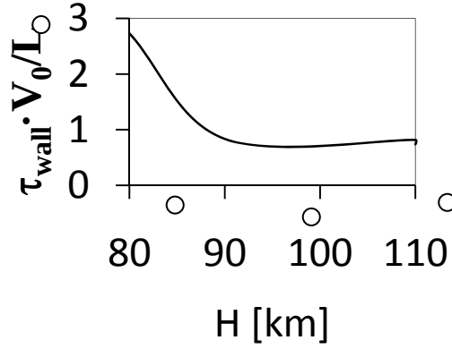
Figure 3. Drag factor for the air breathing Hall thruster: L = 0.5 \text{ m} , r_b = 0.05 \text{ m} , and r_a = 0.03 \text{ m}
