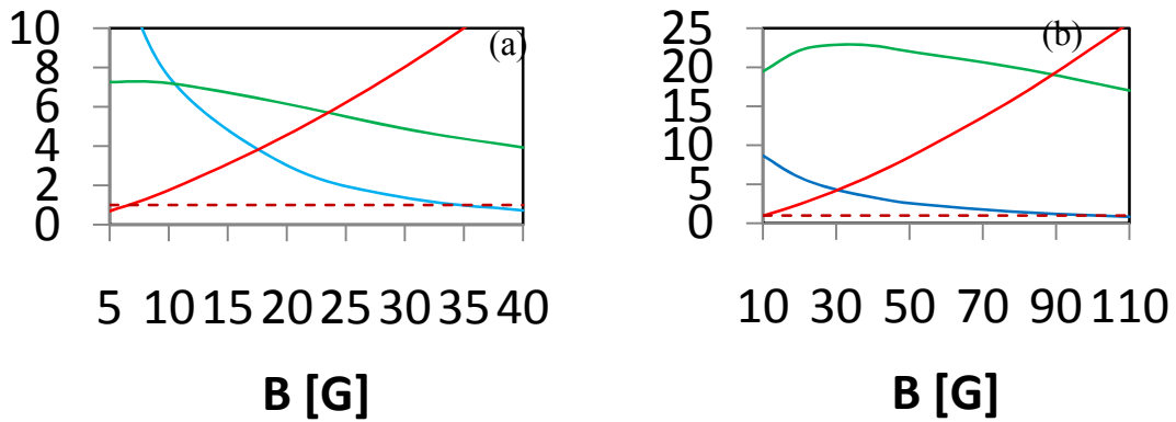
Figure 4. The \tau_0 / \tau_{ioniz} - blue line, \tau_{e-life} / \tau_{ioniz} - green line, (r_b - r_a) / r_L - red line calculated for H = 90 \text{ km} and \varphi = 3 \text{ kV} - (a) and \varphi = 30 \text{ kV} - (b); the broken line correspond to unity.
