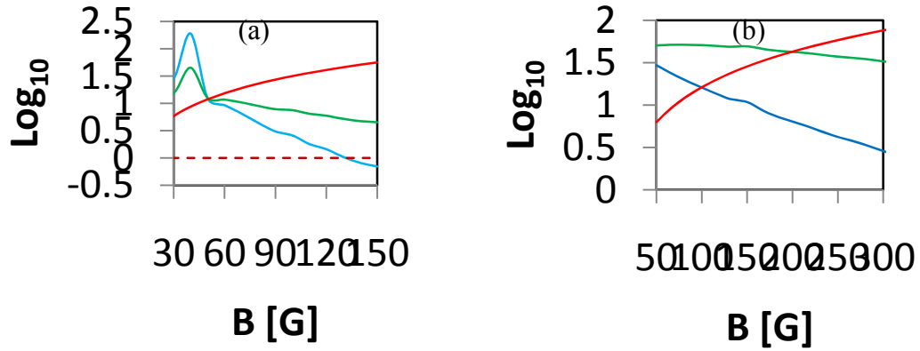
Figure 5. The \tau_0 / \tau_{ioniz} - blue line, \tau_{e-life} / \tau_{ioniz} - green line, (r_b - r_a) / r_L - red line calculated for H = 80 km and \varphi = 3 kV - (a) and \varphi = 30 kV - (b).
