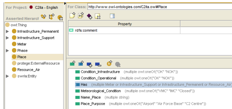
Figure 5 – Local class and attribute
