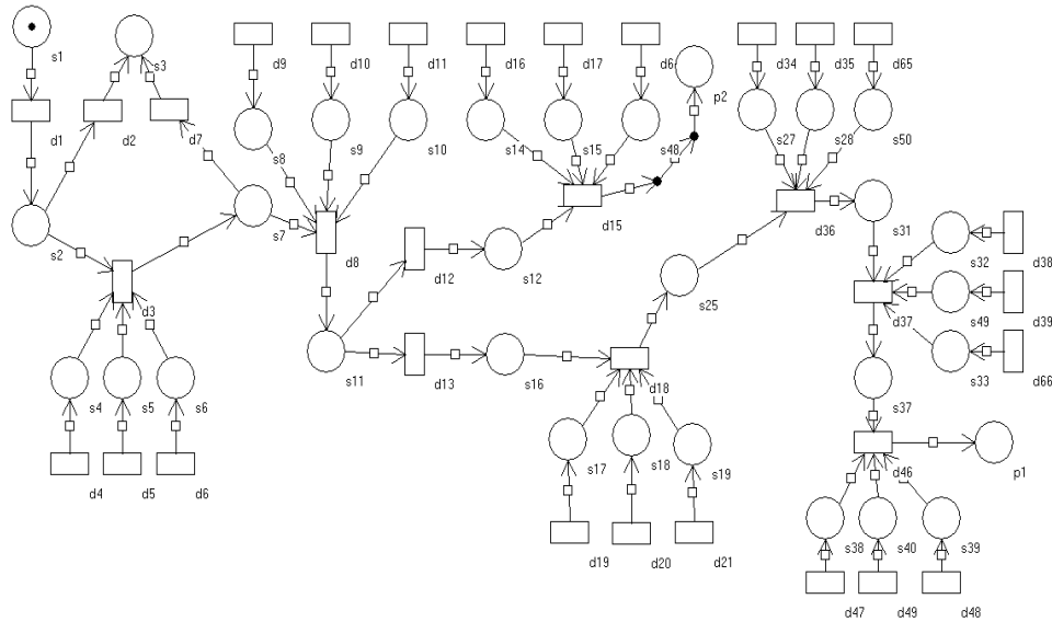
Figure 2 – Part of Air Defense Petri Net [14]
