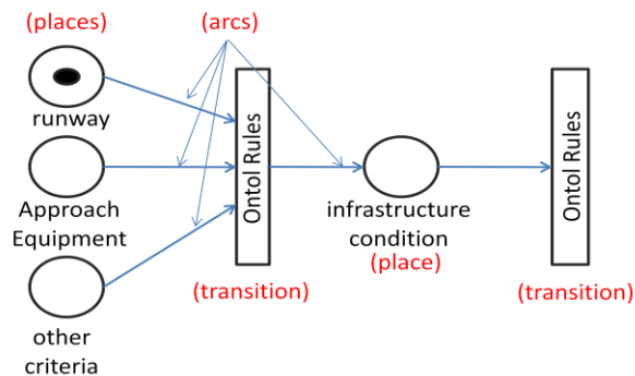
Figure 9 – Infrastructure Conditions Rules
