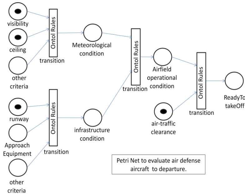
Figure 7 – Petri Net
