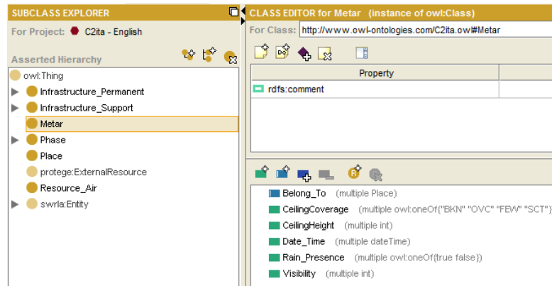
Figure 4 – METAR class and attribute
