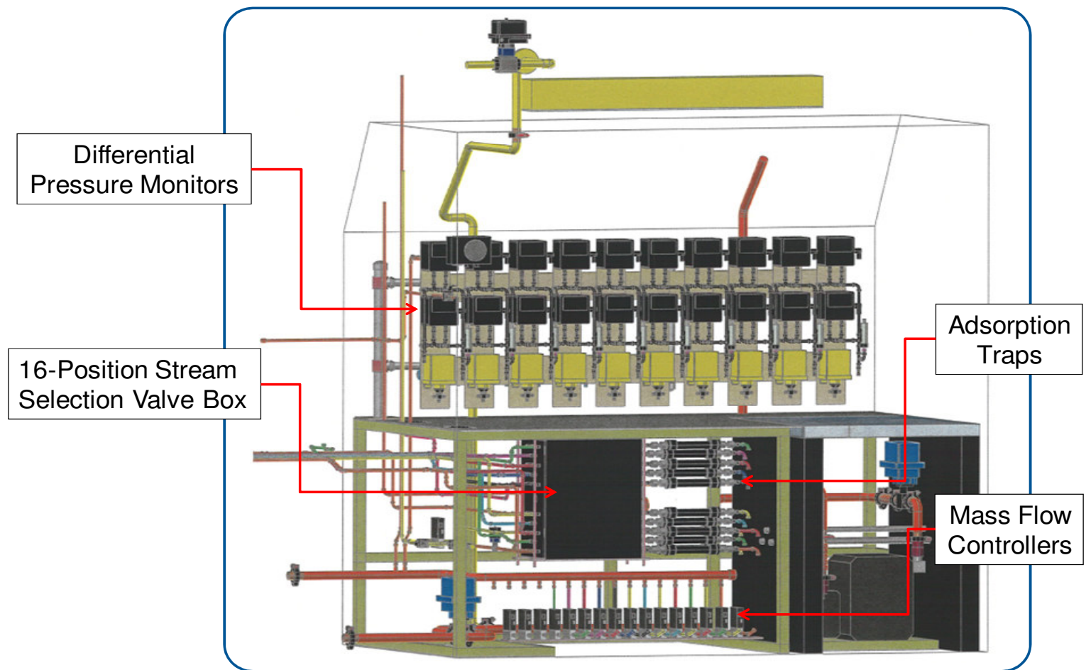
Figure 7. Final CBART Analytical Hood Configuration with Sample Train (as of September 30, 2009)
