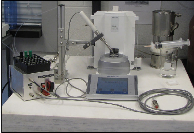
Figure 15. CBART Touchless Dispenser Mounted on an Analytical Balance
