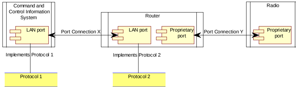
Figure 4: NAF System View 2b – Port Connections
