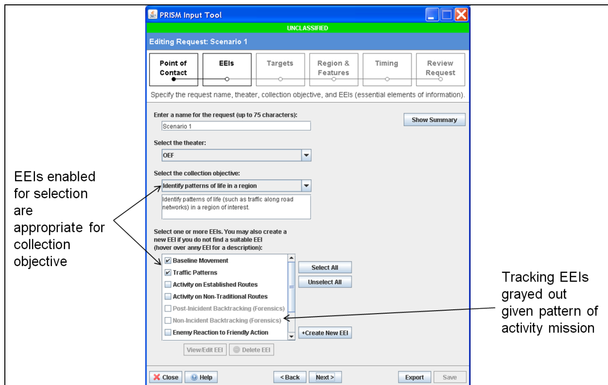
Figure 4: The PRISM Input Tool – Specifying collection objective and EEIs.
