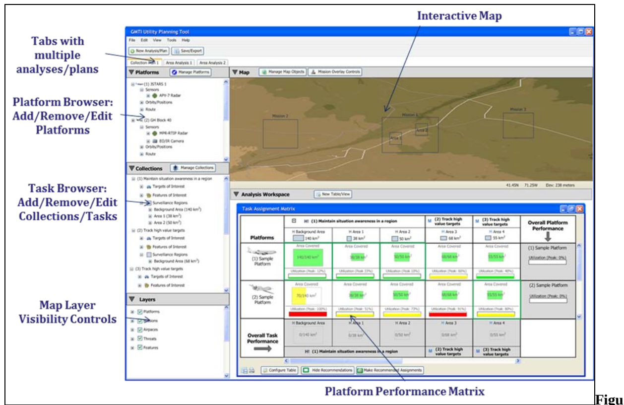
Figure 6: GMTI Planning Tool – Overview.
