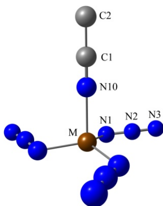
Figure 1. Calculated C_{3h} structure of the acetonitrile adducts \text{M}(\text{N}_3)_3 \cdot \text{CH}_3\text{CN} ( \text{M} = \text{Ga}, \text{In} ). Bond lengths and angles are listed in the Supplementary Material.
