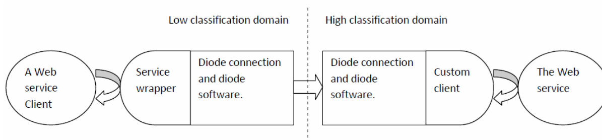
Figure 2: Proof-of-concept architecture
