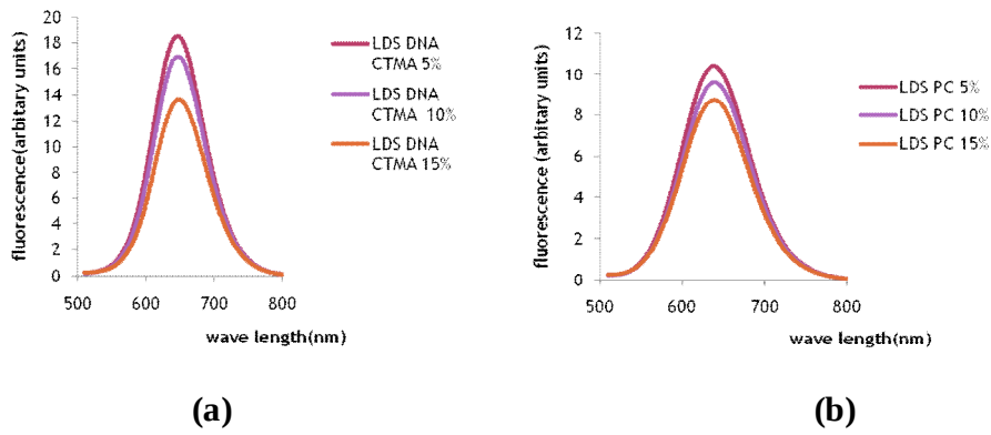
Fig. 22. Thin film fluorescence spectra of DNA-CTMA-LDS698 (a) and PC-LDS698 (b) as function of chromophore concentration.
