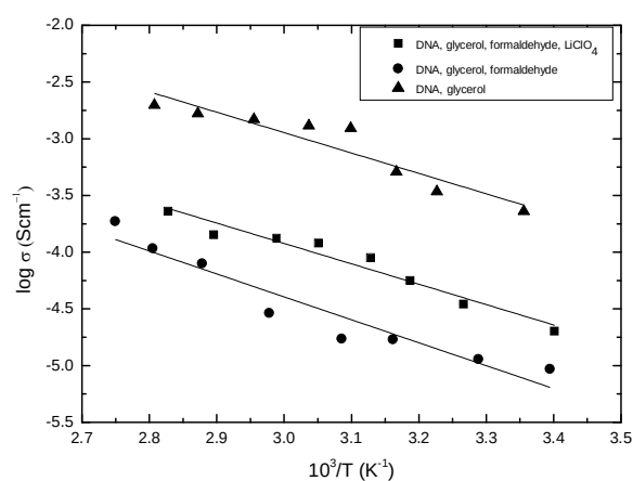
Fig. 24. Arrhenius plot for DNA-based electrolytes for samples plasticized with glycerol: DNA:glycerol A ( \blacktriangle ), DNA:glycerol+formaldehyde (*), DNA:glycerol+formaldehyde ( \blacksquare ).
