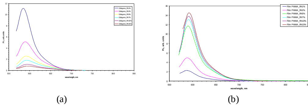
Fig. 21. Thin film fluorescence spectra of collagen-Rh610 (a) and PMMA-Rh610 (b) as function of chromophore concentration.
