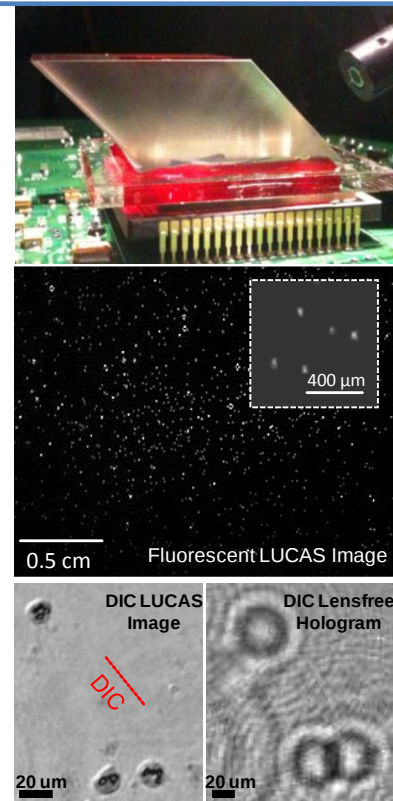
Fig.4 (Top) Ultra-wide field of view (FOV) lensfree on-chip fluorescent imaging set-up. (Middle) High throughput lensfree fluorescent imaging on a chip is illustrated over an FOV of 8.4\text{ cm}^2 for fluorescently labeled cells. [16,18] This lensfree fluorescent image was pumped through an LED and was acquired within an integration time of \sim 1\text{ sec} . The inset image is digitally cropped from the large FOV. The raw lensfree fluorescent images are digitally processed through compressive sampling to achieve a spatial resolution of \sim 10\mu\text{m} over >8\text{ cm}^2 . [16] Dual imaging mode is also demonstrated to enable lensfree transmission holographic imaging and fluorescent imaging of an ultra-wide FOV within the same benchtop LUCAS platform. [18] (Bottom Row) LUCAS based DIC (Nomarski) images of white blood cells are demonstrated. The same holographic microscope of Fig. 1(a) can be converted into a lensless DIC microscope with two polarizers and thin birefringent crystals (e.g., quartz). [10,13] Each birefringent uniaxial crystal creates an ordinary and an extra-ordinary hologram of the cell, which are separated by a shear distance of \sim 1\mu\text{m} from each other. The interference of these holograms codes the DIC information into the cell shadow. [13] Despite the major differences in the way that the lensless holograms are physically created and recorded for regular transmission imaging vs. DIC imaging, the image reconstruction process remains the same in both. [10,13] The shear direction is indicated in the figure with the red dashed line.
