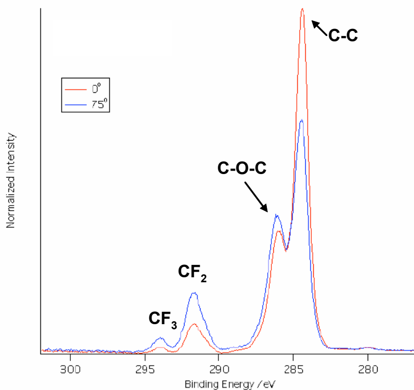
Figure 51. XPS C 1s spectra of the surface of the amphiphilic SABC with ethoxylated fluoroalkyl side chains derived from the \text{PS}_{8\text{K}}\text{-}b\text{-P}(\text{E/B})_{25\text{K}}\text{-}b\text{-PI}_{10\text{K}} precursor polymer spun coat on Si taken at both 0^\circ and 75^\circ incidence angles.
