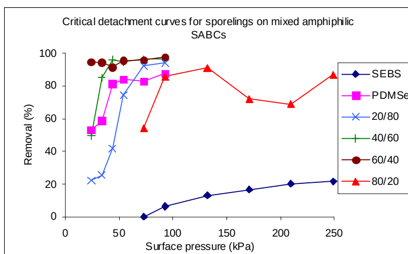
Figure 84. Critical detachment force curves for Ulva sporelings on mixed amphiphilic \text{PS}_{8\text{K}}\text{-}b\text{-P}(\text{E/B})_{25\text{K}}\text{-}b\text{-PI}_{20\text{K}} derived SABCs when exposed to a water jet. Ratios listed are PEG550:F10H10 in the reaction feed.
