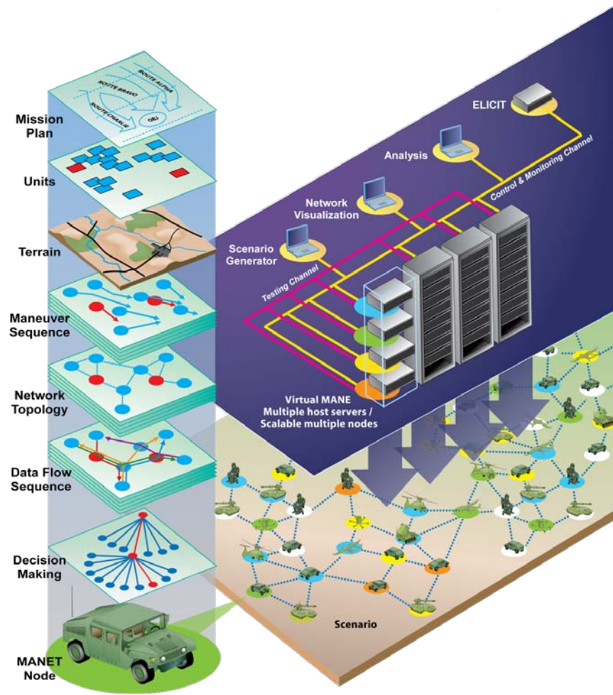
Figure 4. Overview of architecture and modules of the Wireless Emulation Laboratory (WEL)
