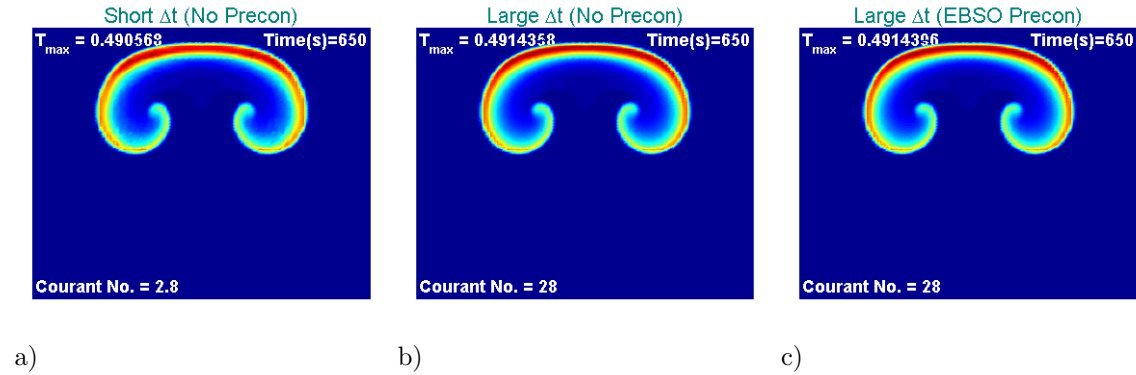
FIGURE 4.5. Perturbation potential temperature fields at 650s from rising thermal bubble problem using a small \Delta t (panel a), a large \Delta t and no preconditioner (panel b), and the same large \Delta t and the EBSO preconditioner. For all runs N_e = 40^2 , and the T_{\max} number in the upper left of each figure gives the warmest temperature at any node in the domain.
