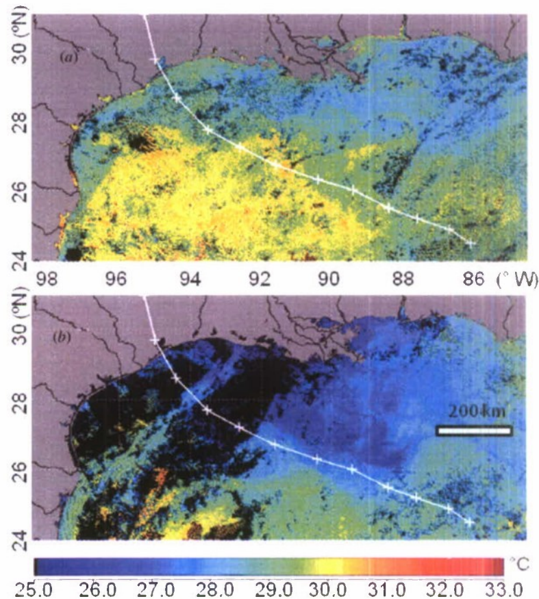
Figure 2. MODIS Terra imagery depicting SST distribution averaged over a 5-day period (a) before (6–10 September) and (b) after (14–18 September) the passage of Hurricane Ike.
