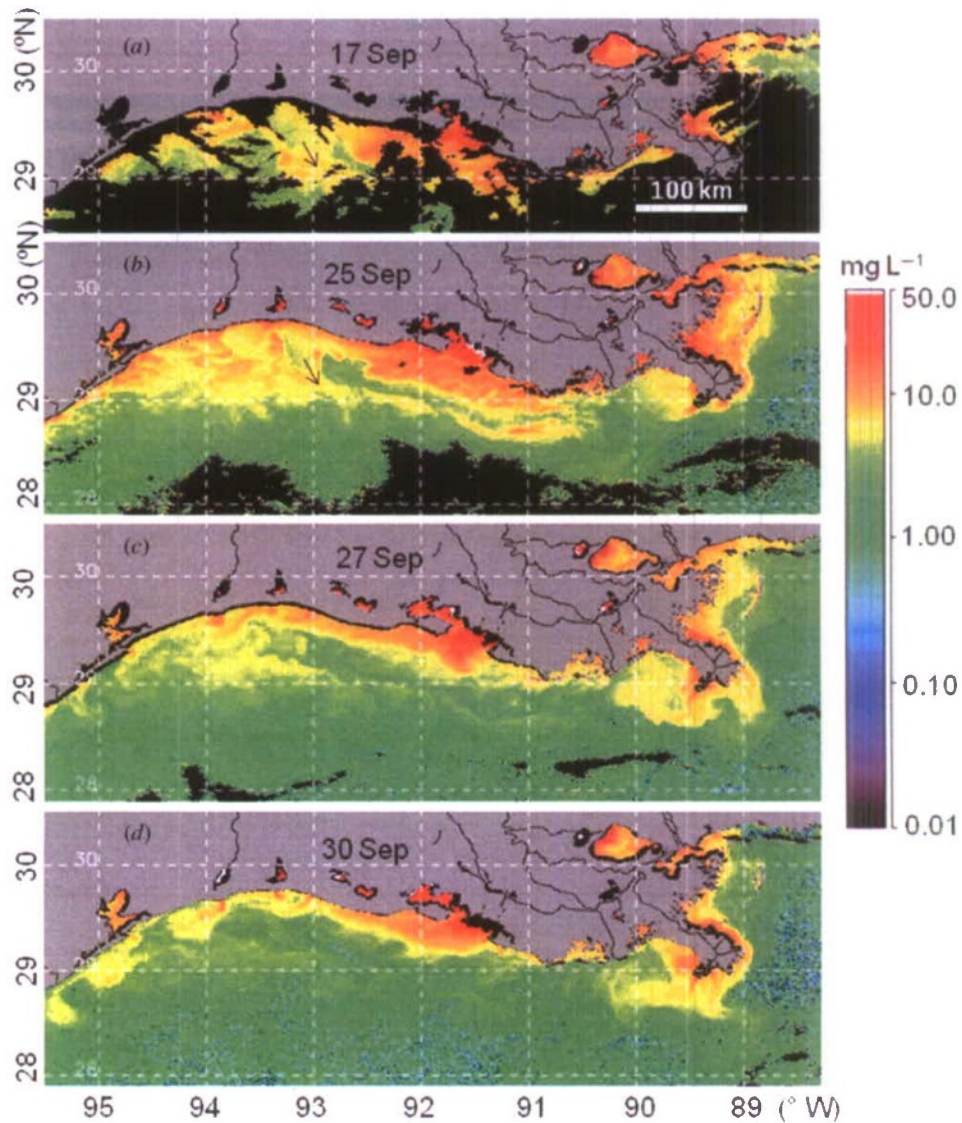
Figure 5. SeaWiFS-derived SPM for (a) 17, (b) 25, (c) 27 and (d) 30 September 2008. Arrows indicate the location of the elevated SPM bands.
