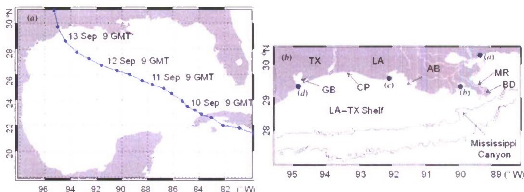
Figure 1. (a) Track of Hurricane Ike in the Gulf of Mexico. (b) Mississippi–Louisiana–Texas (MsLaTex) shelf showing the bathymetry, the location of tide gauges and the domain of the MsLaTex nested NCOM model. Tide gauge locations are labelled as (a) Bay Waveland Yacht Club, MS; (b) Grande Isle, LA; (c) Freshwater Canal Locks, LA; (d) Galveston Pleasure Pier, TX. The abbreviations are as follows: TX, Texas; LA, Louisiana; AB, Atchafalaya Bay; CP, Calcasieu Pass; GB, Galveston Bay; MR, Mississippi River; BD, birdsfoot delta.
