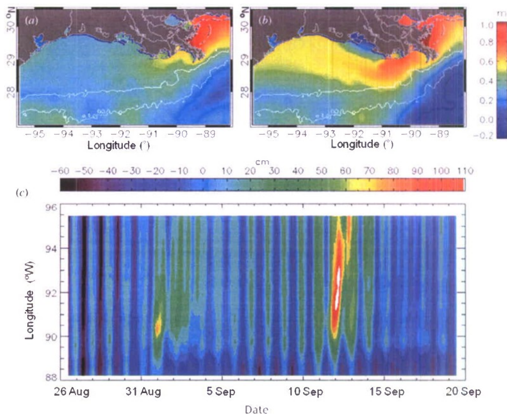
Figure 4. NCOM SSH on (a) 11 September at 1200 UTC and (b) 12 September at 0600 UTC. (c) Time–distance plot of NCOM SSH along the 28.5°N latitude.
