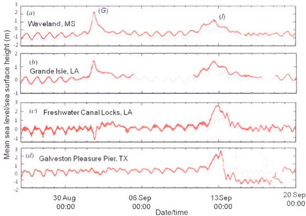
Figure 3. (a)–(d) Mean sea level (MSL) from NOAA stations (solid lines) and sea surface height (SSH) from NCOM (dotted lines) along the Louisiana–Texas coast corresponding to locations shown in figure 1(a). (G) and (I) denote storm surge events due to Hurricanes Gustav and Ike.
