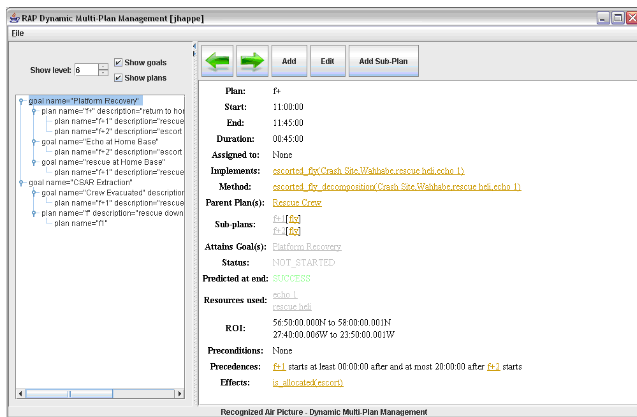
Figure 9 The Browser View, Showing a Plan and its HTN Task and Method
