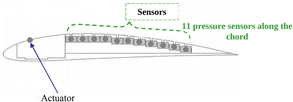
Figure 18. NACA 4412 Airfoil
