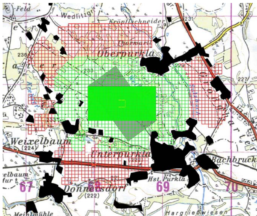
Figure 11: Determination of visibility zones and fire zones based on a given position area. Green cells indicate visible areas which can also be reached by direct fire (i.e. with the given type of weapon system). Red cells indicate areas which are still visible but cannot be reached by fire. Given the center of the position area (green rectangle) other alignments (grey rectangle) are possible. The consideration of different possible alignments may extend the calculated zones.
