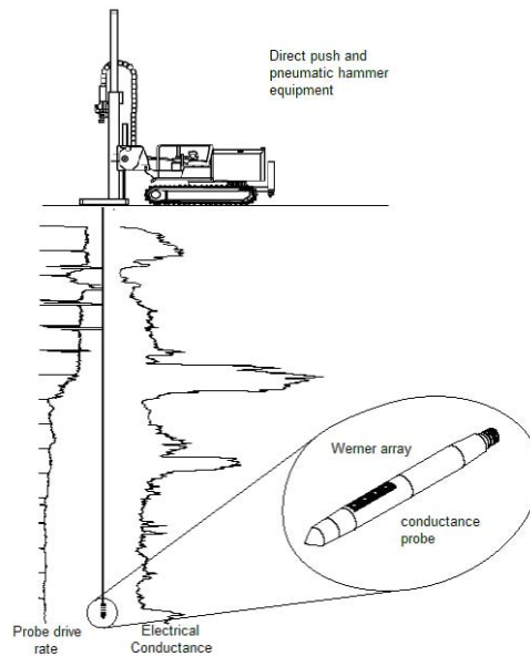
Figure 3. Direct push drilling unit, Electrical Conductance probe, and example profile. Most recently, HRST K estimates were collected in numerous wells that were fully screened through the aquifer material (Ross, 2004; Ross and McElwee, 2007). These independent studies and the research presented here produced estimates of K that can be collected into a database. After compiling these data, vertical and lateral variations of the K distribution are evident. Typically at GEMS, K increases with depth in the sands and gravels, and low K material can be associated with high EC measurements, usually associated with the overlying silt and clay sediments. In most areas at GEMS, “layers” or zones of high K material are apparent in the sand and gravel aquifer.
