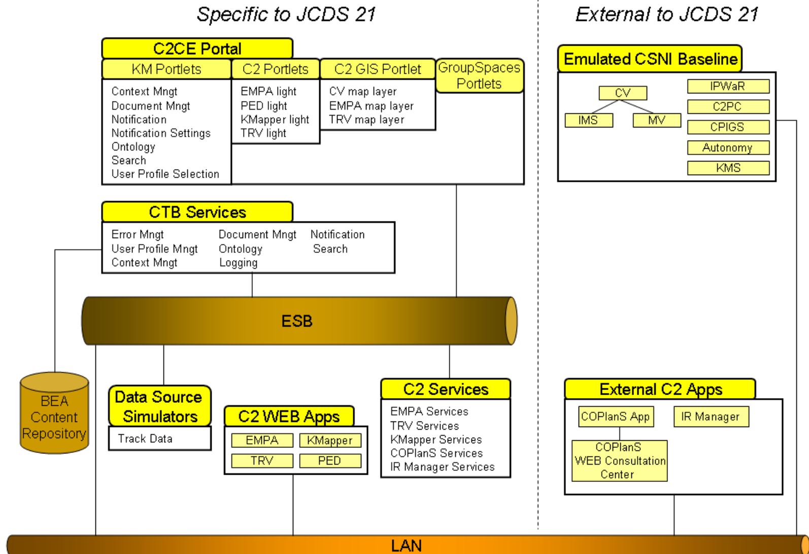
JCDS 21 Service-Oriented Architecture (SOA)
