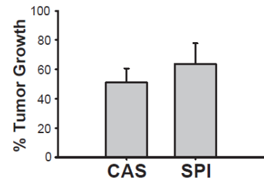
Figure 2. Tumor growth represents the percentage change in tumor volume during 2 weeks after initial detection. No significant changes in tumor growth rate were observed for tumors detected in Wnt-Tg mice fed CAS (n= 16) compared to SPI (n=10).
