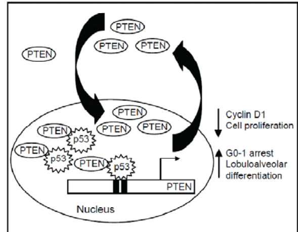
Figure 1. In the presence of GEN, the nuclear pool of PTEN is increased leading to increased levels of nuclear p53, promotion of PTEN/p53 complex formation, increased recruitment of the PTEN/p53 complex, and hence activation of PTEN transcription. A functional outcome of increased nuclear PTEN is the reduction in the expression of pro-proliferative genes cyclin D1 and pleiotrophin, resulting in G0-1 arrest and leading to early lobuloalveolar differentiation (Adapted from Rahal and Simmen, 2010).
