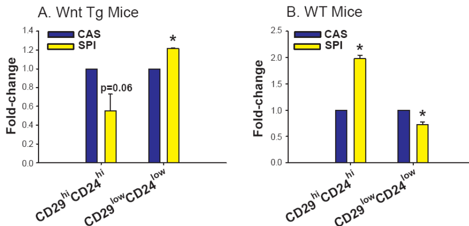
Figure 3 (left). FACS analysis of MECs in preneoplastic mammary glands of Wnt-Tg mice (A) or adult WT mice (B) using mouse mammary stem cell markers (CD24 and CD29) in the lineage negative population (CD45 - , TER119 - , and CD31 - ). * = P<0.05 relative to CAS diet. Data shown is at least from 3 independent experiments (n=5-7 mice per experiment, per diet).
