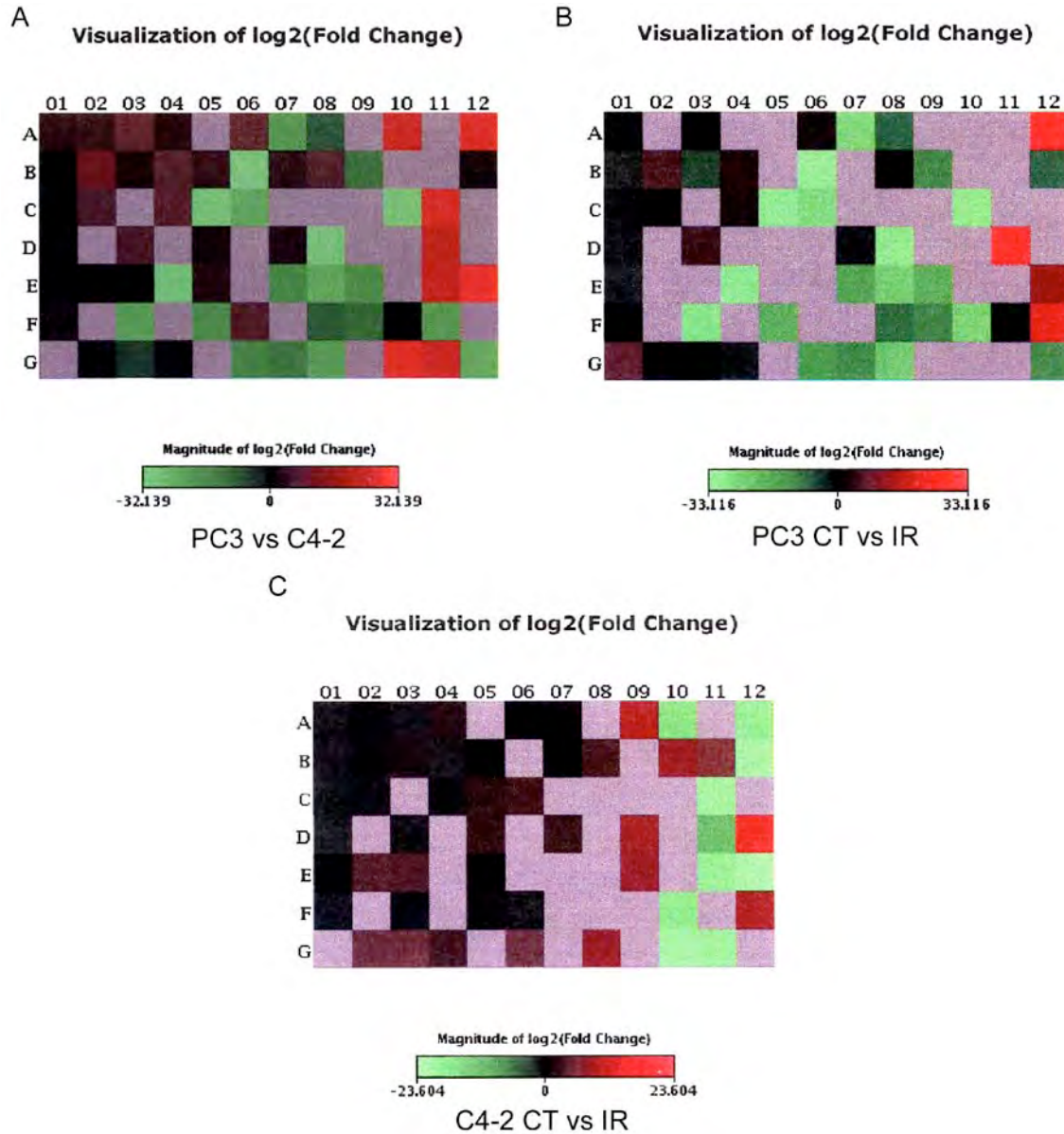
Figure 1. Heat map showing changes in mRNA expression of autophagy regulatory genes following IR using a real time PCR array. (A) Autophagy gene expression comparison between PC3 and C4-2 cells. (B and C) Autophagy gene expression in PC3 and C4-2 cells at 6 hours following irradiation (10 Gy). Fold change normalized to six different housekeeping controls was determined using a web based software tool available from SA Bioscience.
