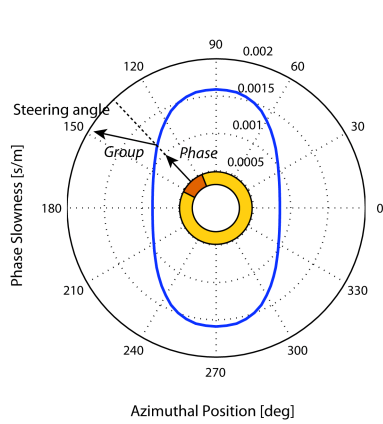
Fig. 6(a): Slowness diagram for unidirectional plate indicating steering angle when waves are launched at a direction of 45^\circ .
