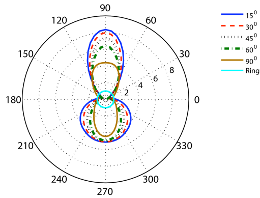
Fig. 3: CLoVER transducer offers increased displacement amplitudes relative to a similarly sized ring transducer for similar electric input (results normalized by the displacement amplitude for a ring geometry; transducer centerline along 90^\circ direction).
