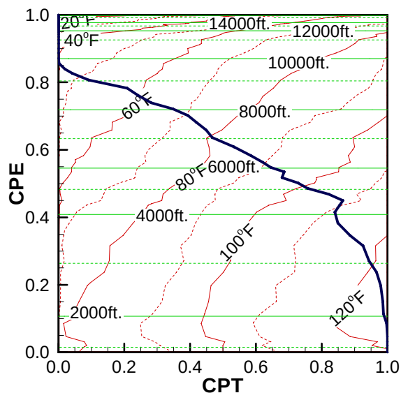
Figure 4: Hover performance ceiling for Afghanistan, based upon mean maximum temperature and geophysical elevation data.
