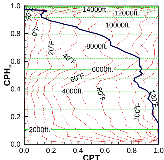
Figure 3: Hover performance ceiling for Afghanistan, based upon combined temperature and equivalent pressure altitude data.
