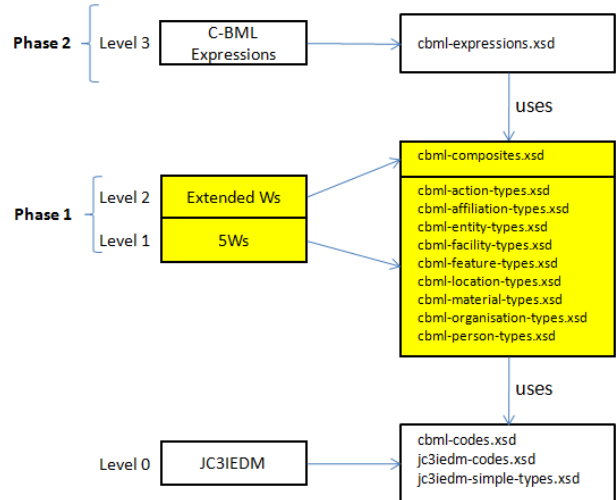
Figure 6- C-BML Layers
