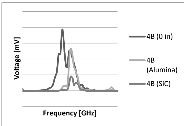
Figure 8. The effects of Alumina and SiC on the performance of the MTJ detector with CPW antenna.
