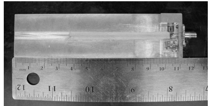
Figure 4. Spintronics passive microwave MTJ detector with coplanar waveguide antenna.
