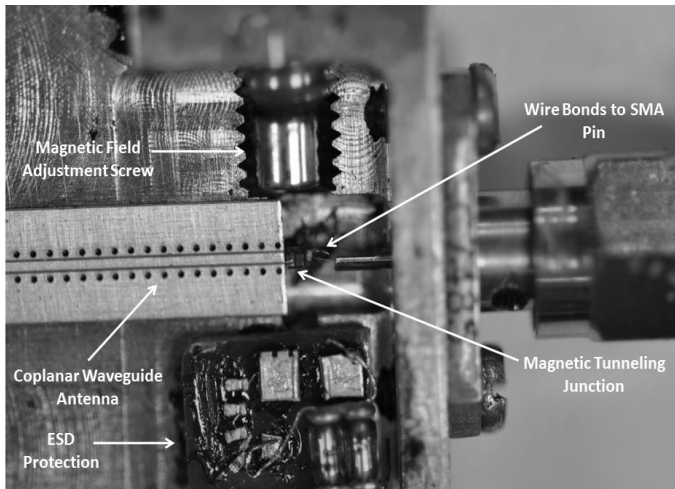
Figure 5. Enlarged view of the spintronics microwave MTJ detector with CPW antenna.
