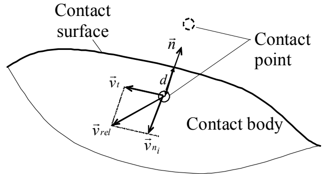
Figure 6. Contact surface and contact node.
