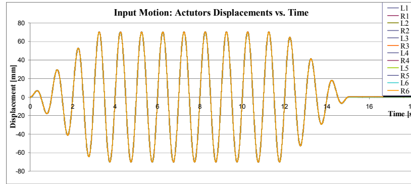
Figure 13. Input motion: harmonic shake 1.0 Hz 70 mm.
