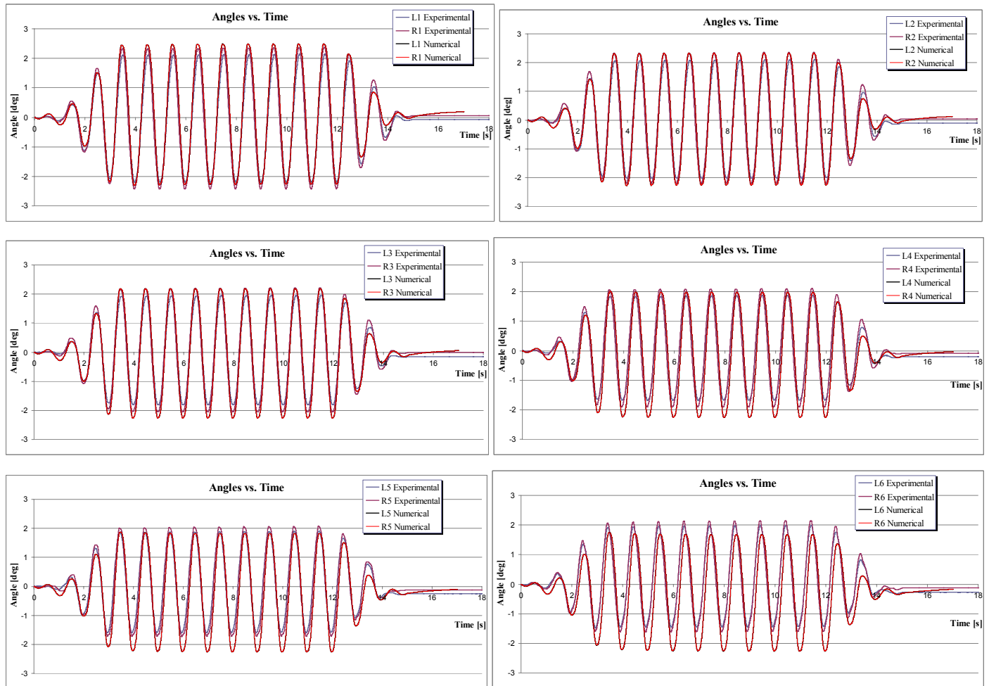
Figure 14. Experiment and simulation angles of the road arms versus time for input motion: harmonic shake 1.0 Hz 70 mm.
