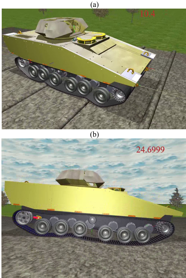
Figure 21. Snapshots of the motion of the tracked vehicle with a continuous belt track. The track is modeled using brick elements for modeling the belt rubber and thin beam elements for modeling the reinforcements. (a) vehicle going over semi-circular bumps; (b) vehicle going over a rough course.
