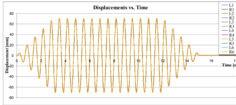
Figure 15. Input motion: harmonic shake 1.5 Hz 70 mm.
