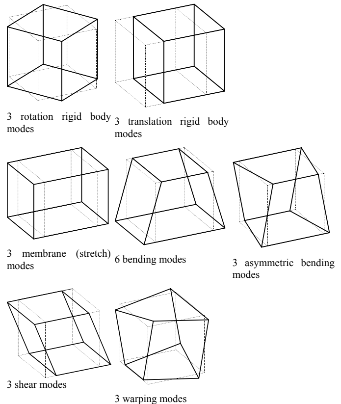
Figure 4. 24 rigid body and deformation modes of a spatial 8-node brick element.
