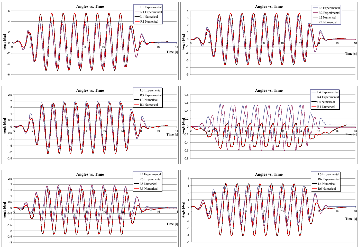
Figure 18. Experiment and simulation angles of the road arms versus time for input motion: harmonic pitch 0.8 Hz 70 mm.
