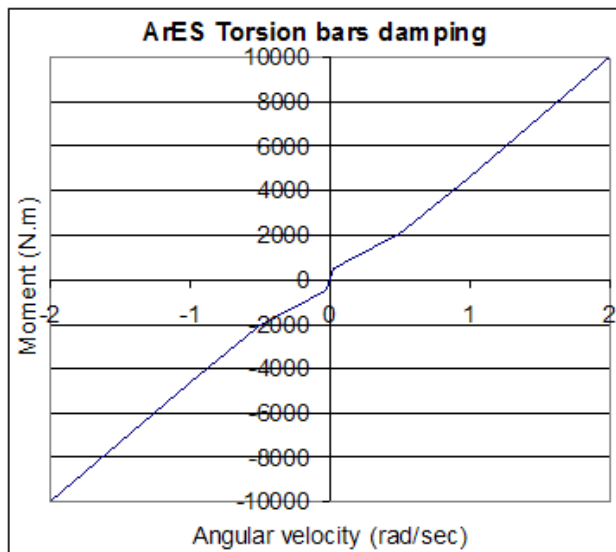
Figure 12. Damping moment versus angular velocity for the torsion bars.
