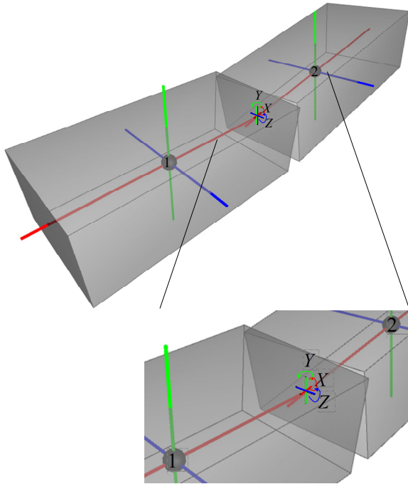
Figure 3. Spatial lumped parameters 2-node beam element. Each node is modeled as a rigid body. The X, Y, Z local axes of each node are shown red, green and blue, respectively. The element consists of 3 truss elements (for modeling the axial and shear response) and 3 torsional spring elements (for modeling the bending and torsion response) located at the center point of the element.
