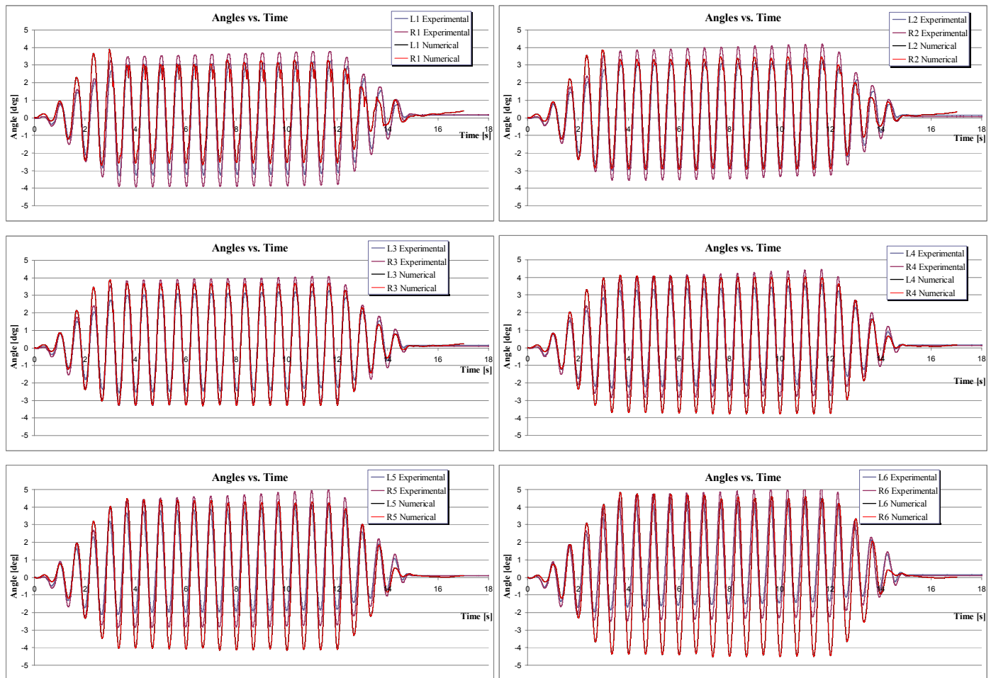
Figure 16. Experiment and simulation angles of the road arms versus time for input motion: harmonic shake 1.5 Hz 70 mm.
