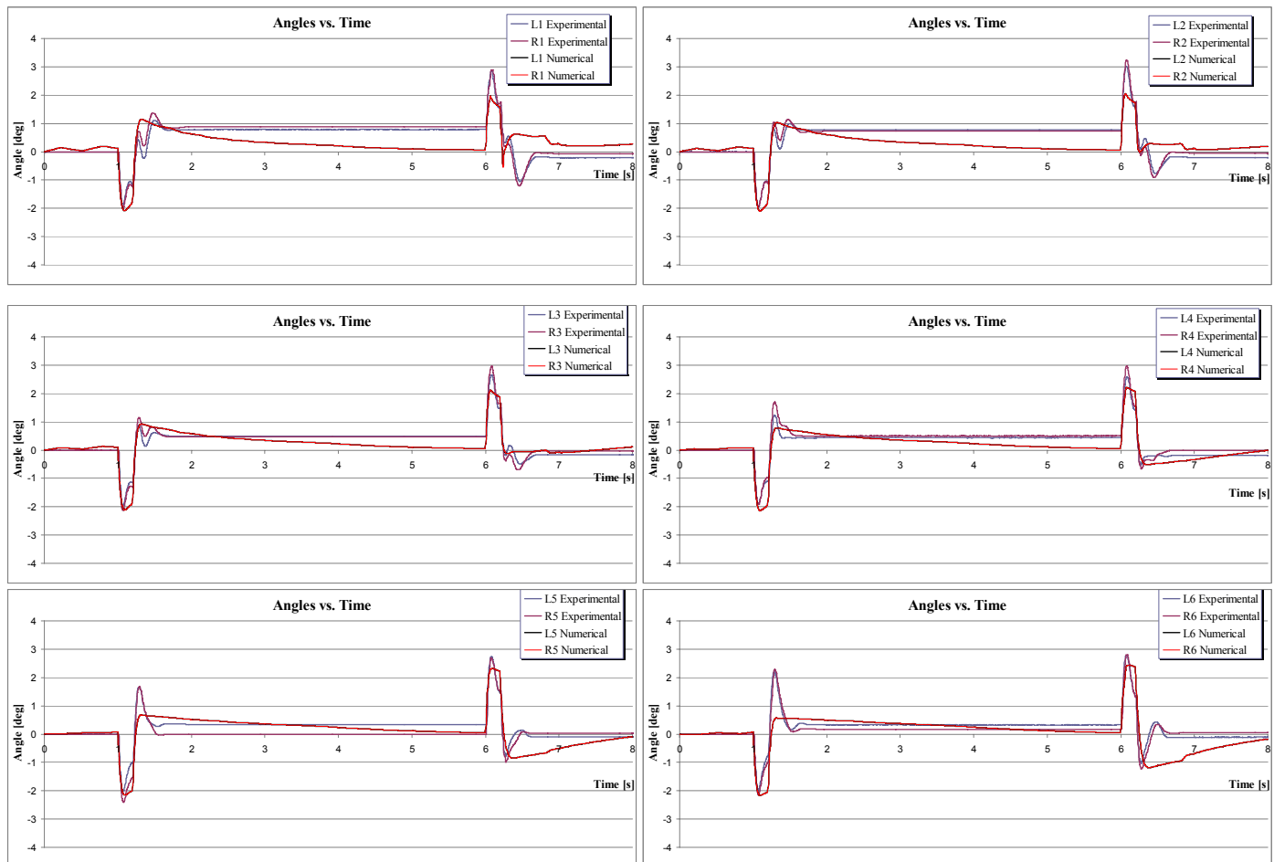
Figure 20. Experiment and simulation angles of the road arms versus time for input motion: ramp shake 90 mm.
