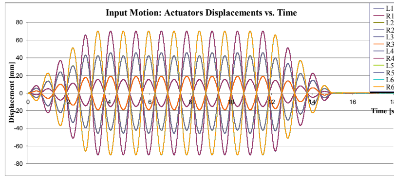
Figure 17. Input motion: harmonic pitch 0.8 Hz 70 mm.
