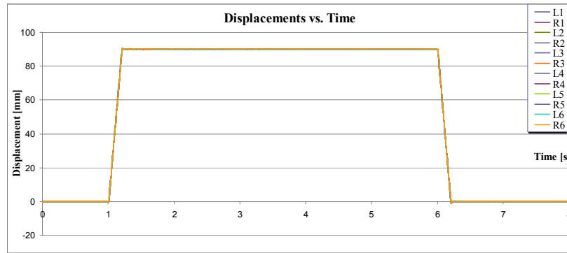
Figure 19. Input motion: ramp shake 90 mm.
