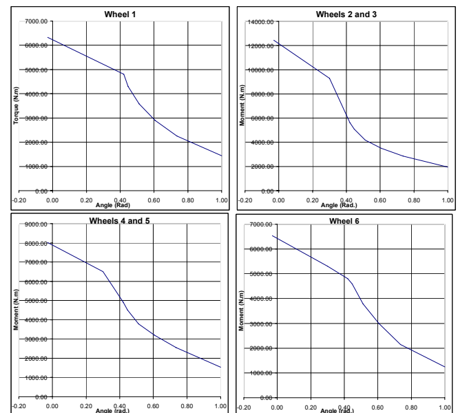
Figure 11. Experimentally measured rotational stiffness (torque versus angle) of the torsion bar at each road wheel.
