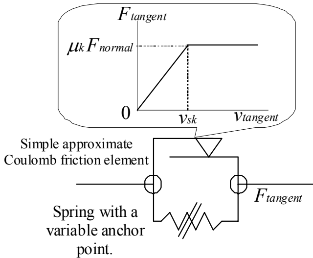
Figure 7. Asperity spring friction model.
