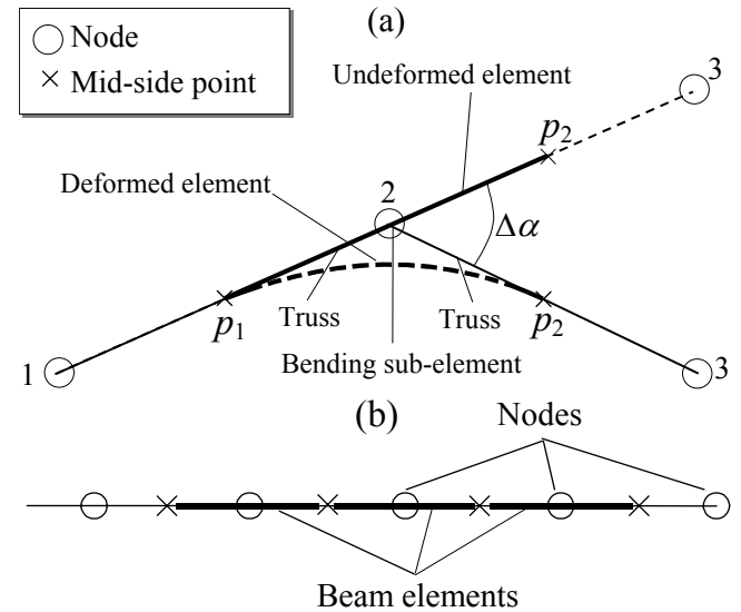
Figure 2. (a) 3-noded beam element; (b) finite element discretization of a beam using the 3-noded beam element.
