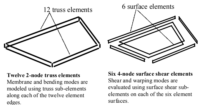
Figure 5. Sub-elements of the 8-node lumped-parameters brick element.
