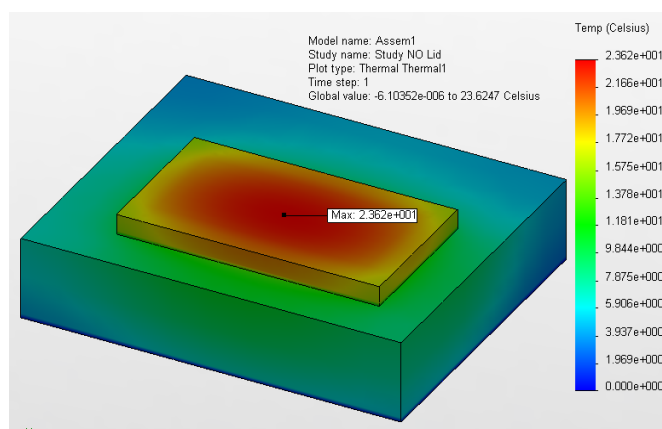
Figure 12: Thermal Analysis Model
