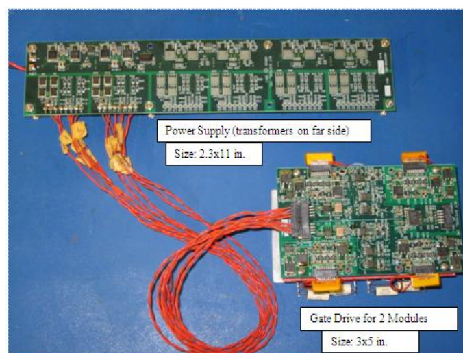
Figure 8: Prototype Gate Drive and Power Supply Hardware for Thermal Evaluation
