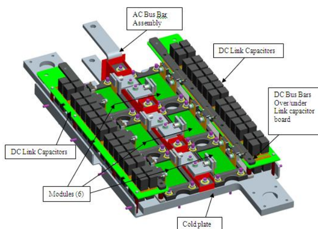
Figure 13: Cold Plate Components, Top View
