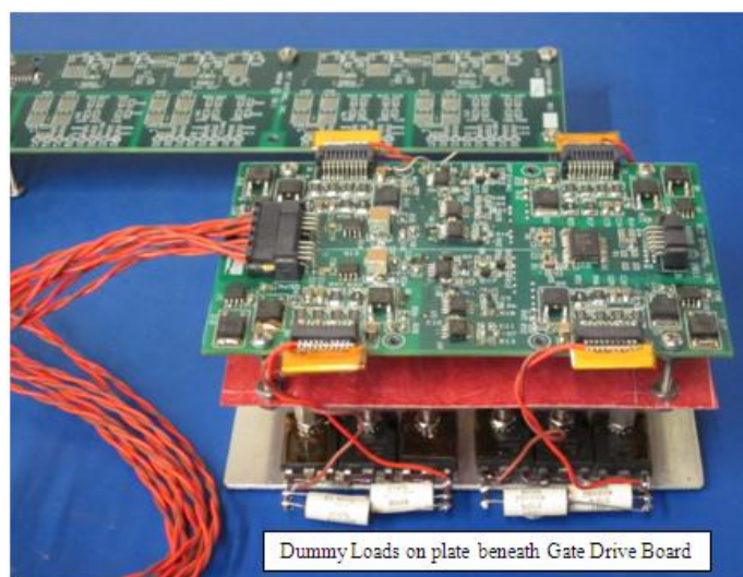
Figure 9: Prototype Gate Drive Hardware With Dummy Loads for Thermal Evaluation
