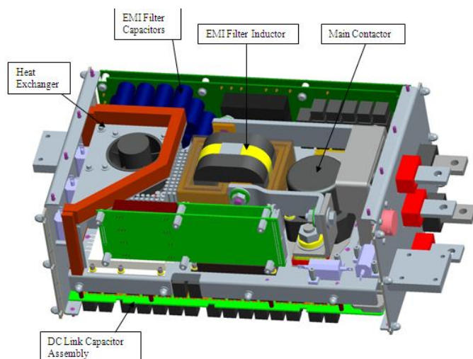
Figure 14: Motor Drive Package, Internal, Bottom View
