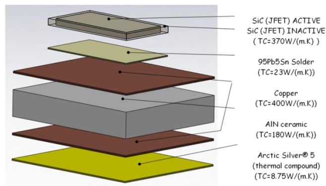
Figure 11: Stack-up for Thermal Analysis
