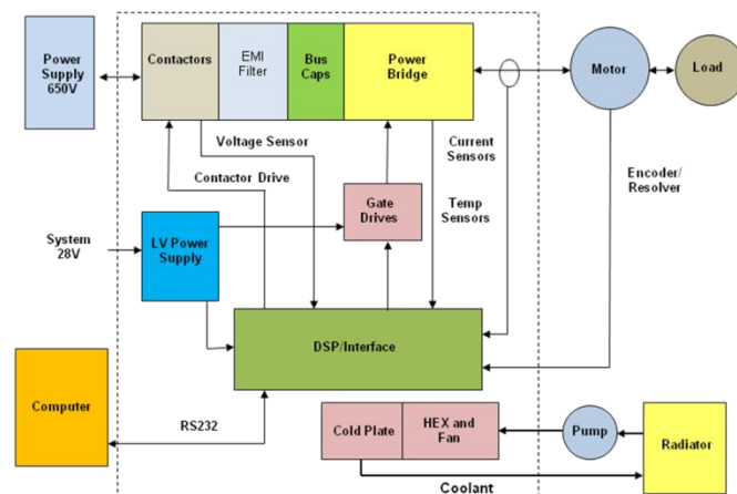
Figure 2: Traction Motor Drive Block Diagram
