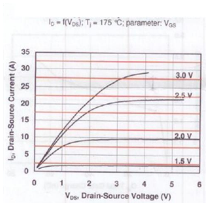
Figure 4: JFET Transconductance Characteristics
