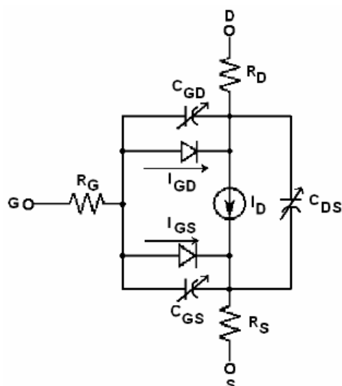
Figure 3: JFET Equivalent Circuit
