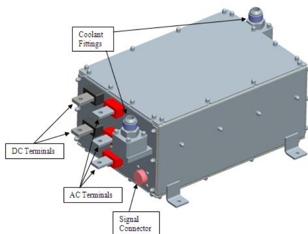
Figure 15: Motor Drive Package, External
