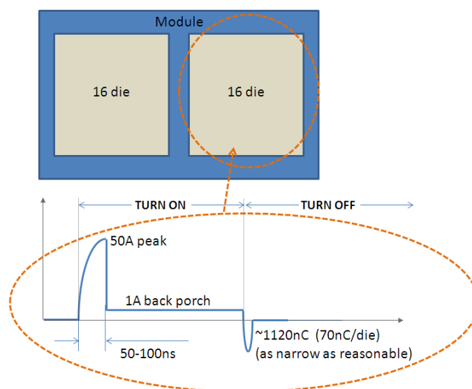
Figure 5: Module Switching Characteristics
