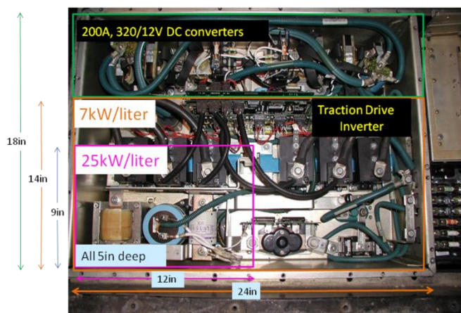
Figure 1: Power Density Comparison between Commercial Drive and TARDEC Requirements
