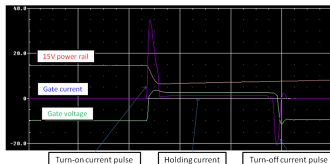
Figure 7: Simulated Gate Drive Circuit Waveforms
