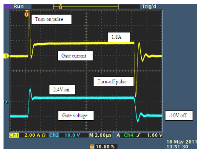
Figure 10: Measured Prototype Gate Drive Waveforms
