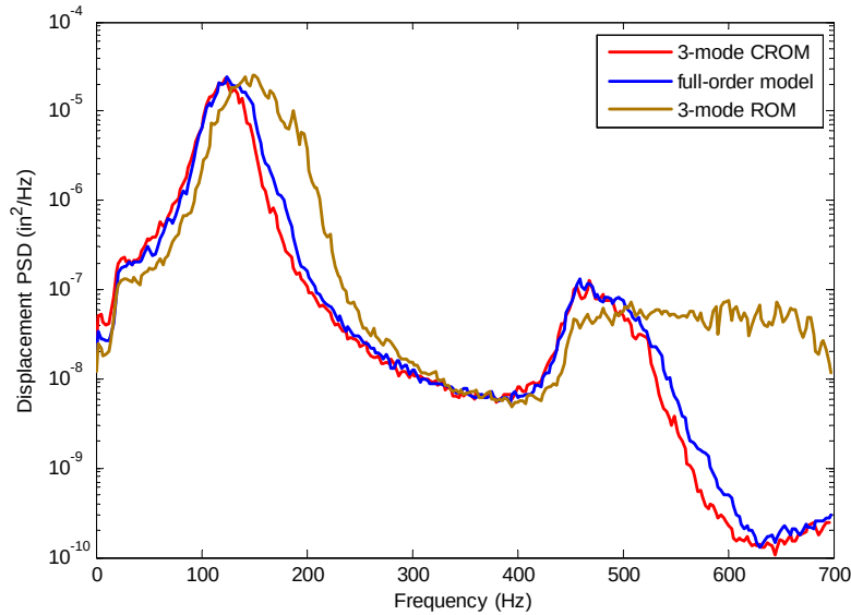
Figure 171. Beam center displacement PSD from nonlinear simulation with direct loading of a three-mode CROM, the full-order model, and a three-mode ROM at 152dB
