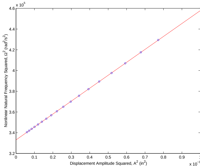
Figure 12. Frequency and amplitude estimates for a set of free response data from Case A (circles) and a linear curve fit through the estimates (solid).
