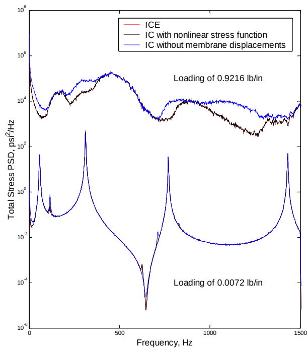
Figure 32. Total stress from various implementations of the IC method.
