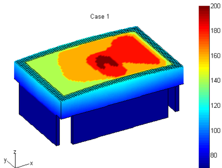
Figure 151. Temperature distribution (°F) for the FEM and ROM for the +110 °F case
