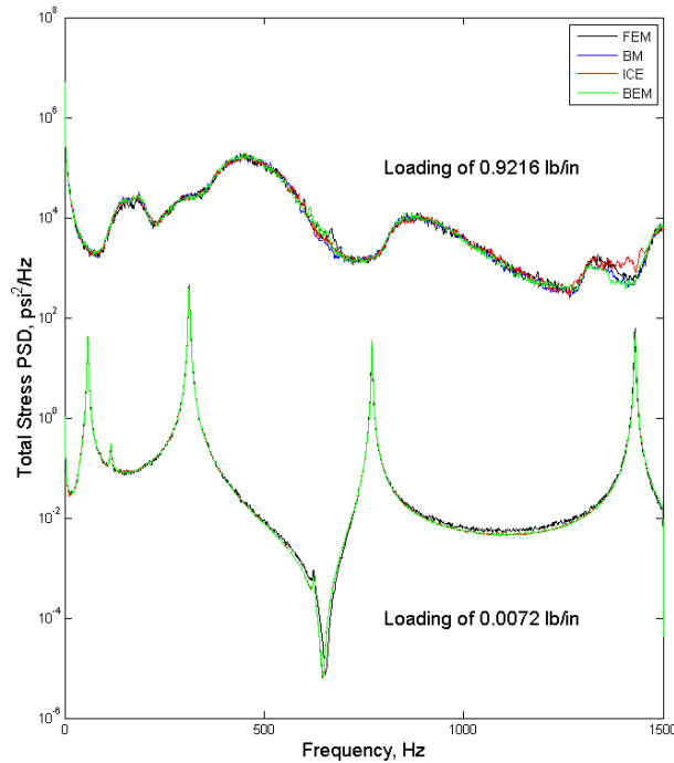
Figure 30. Total stress at the top of the beam, 3.625" from the clamped end.
