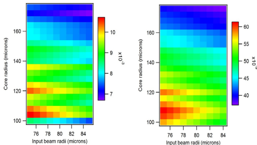
Fig. 22 a) THz power as a function of input beam radius and waveguide core radius (power is in W). The input powers were 100W each. b) THz pulse output energy as a function of input beam radius and waveguide core radius (energy is in J). The input pulse energies were 50 \mu J in 10 nsec pulses (FWHM). Both simulations used a 1 cm interaction length.
