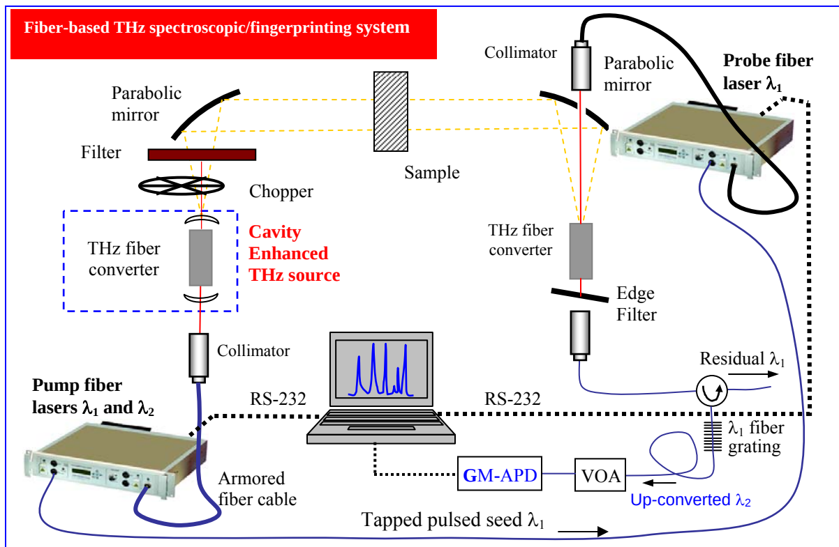
Fig. 1 Schematic of the proposed fiber-based, compact, tunable, THz spectroscopic/fingerprinting system with ultra-high resolution ( < 1 \text{ MHz} ), high sensitivity and room temperature operation.
