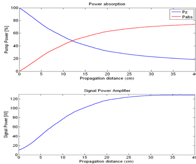
Fig. 12 Simulation of the power performance for the designed LCF to be used as amplifier fiber with 40 cm length.
