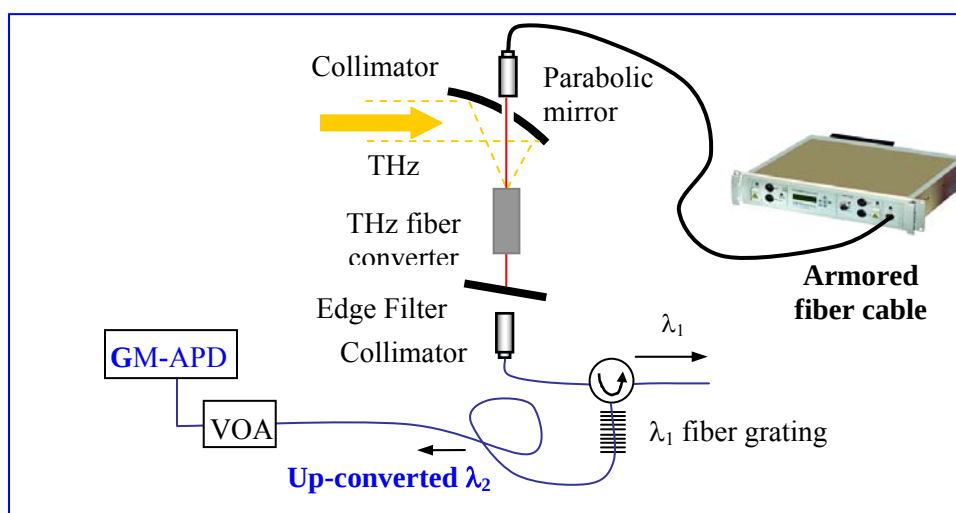
Fig. 30 Fiber-based THz detector based on THz parametric upconversion.
